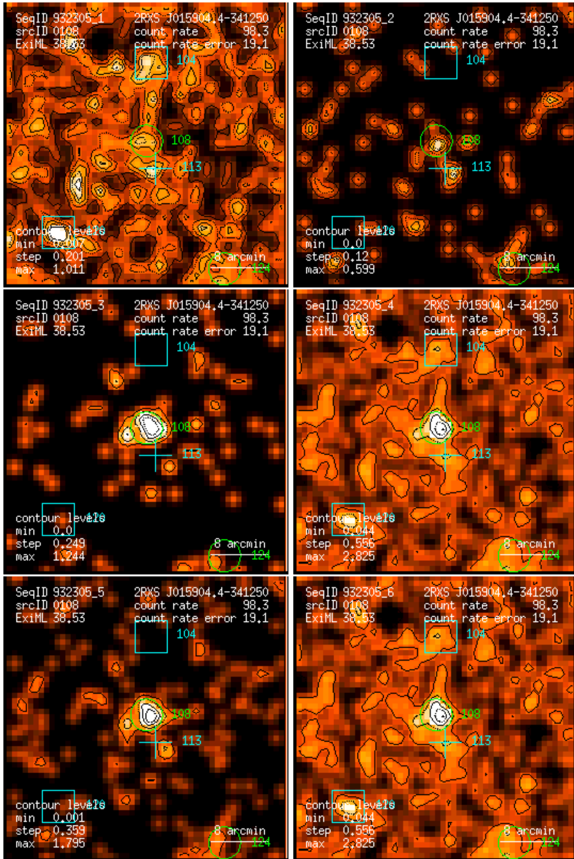
Figure 108: RASS 932305: detection 0108: band rate images, Gaussian filter: (1) PSPC channels 11 – 41, (2) 52 – 90, (3) 91 – 201, (4) 11 – 235, (5) 52 – 201, (6) 11 – 201. Broad band rates in counts/ks. Band rate contour levels in counts/ks/arcmin 2 .
