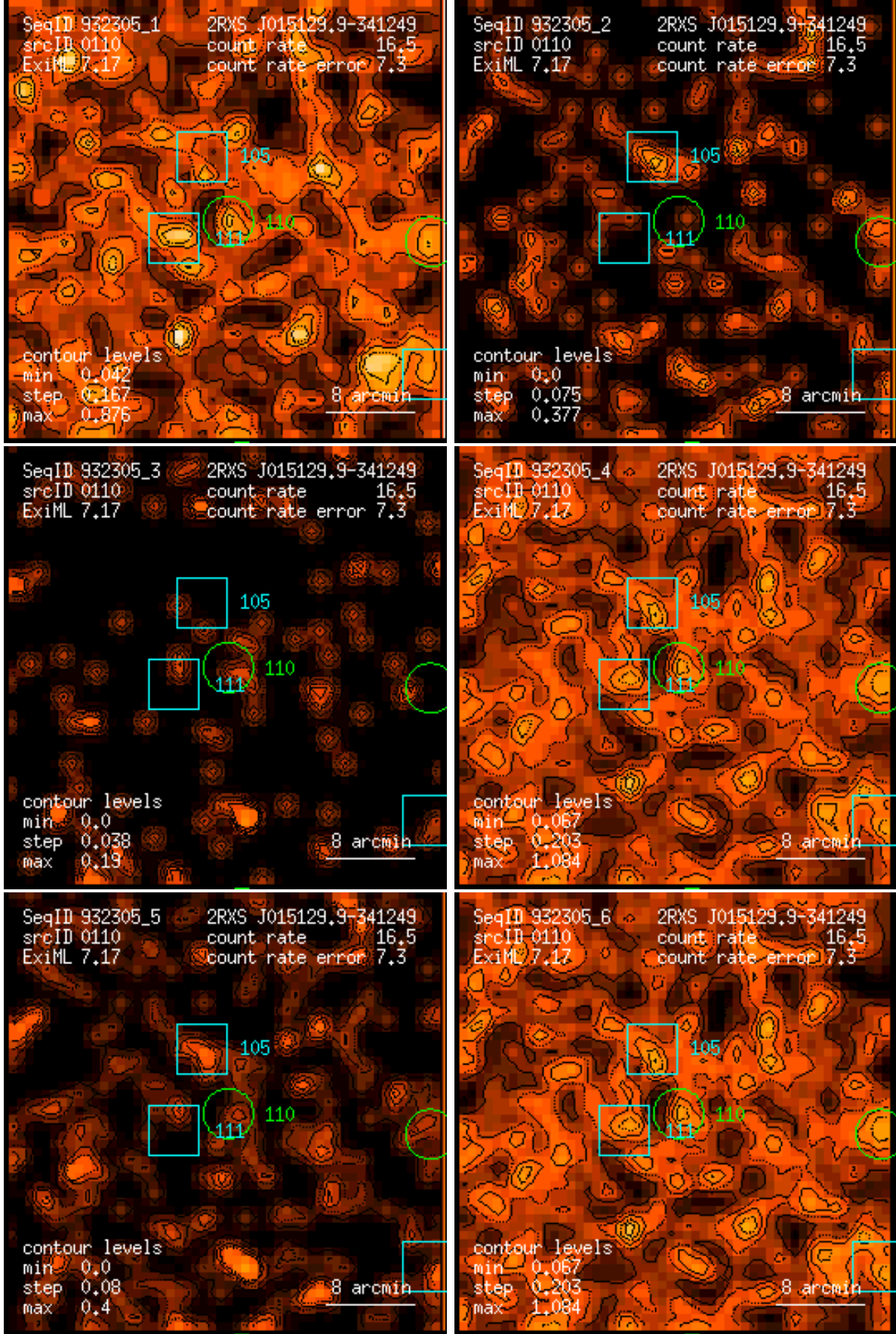
Figure 110: RASS 932305: detection 0110: band rate images, Gaussian filter: (1) PSPC channels 11 – 41, (2) 52 – 90, (3) 91 – 201, (4) 11 – 235, (5) 52 – 201, (6) 11 – 201. Broad band rates in counts/ks. Band rate contour levels in counts/ks/arcmin 2 .
