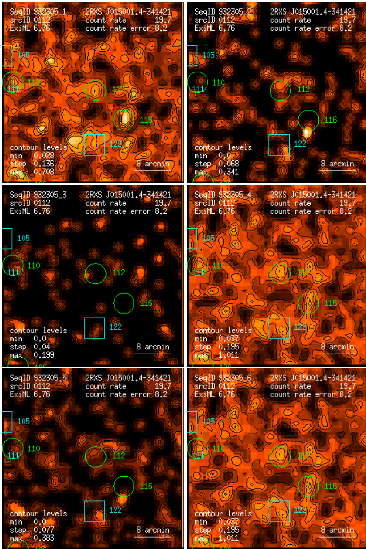
Figure 112: RASS 932305: detection 0112: band rate images, Gaussian filter: (1) PSPC channels 11 – 41, (2) 52 – 90, (3) 91 – 201, (4) 11 – 235, (5) 52 – 201, (6) 11 – 201. Broad band rates in counts/ks. Band rate contour levels in counts/ks/arcmin 2 .
