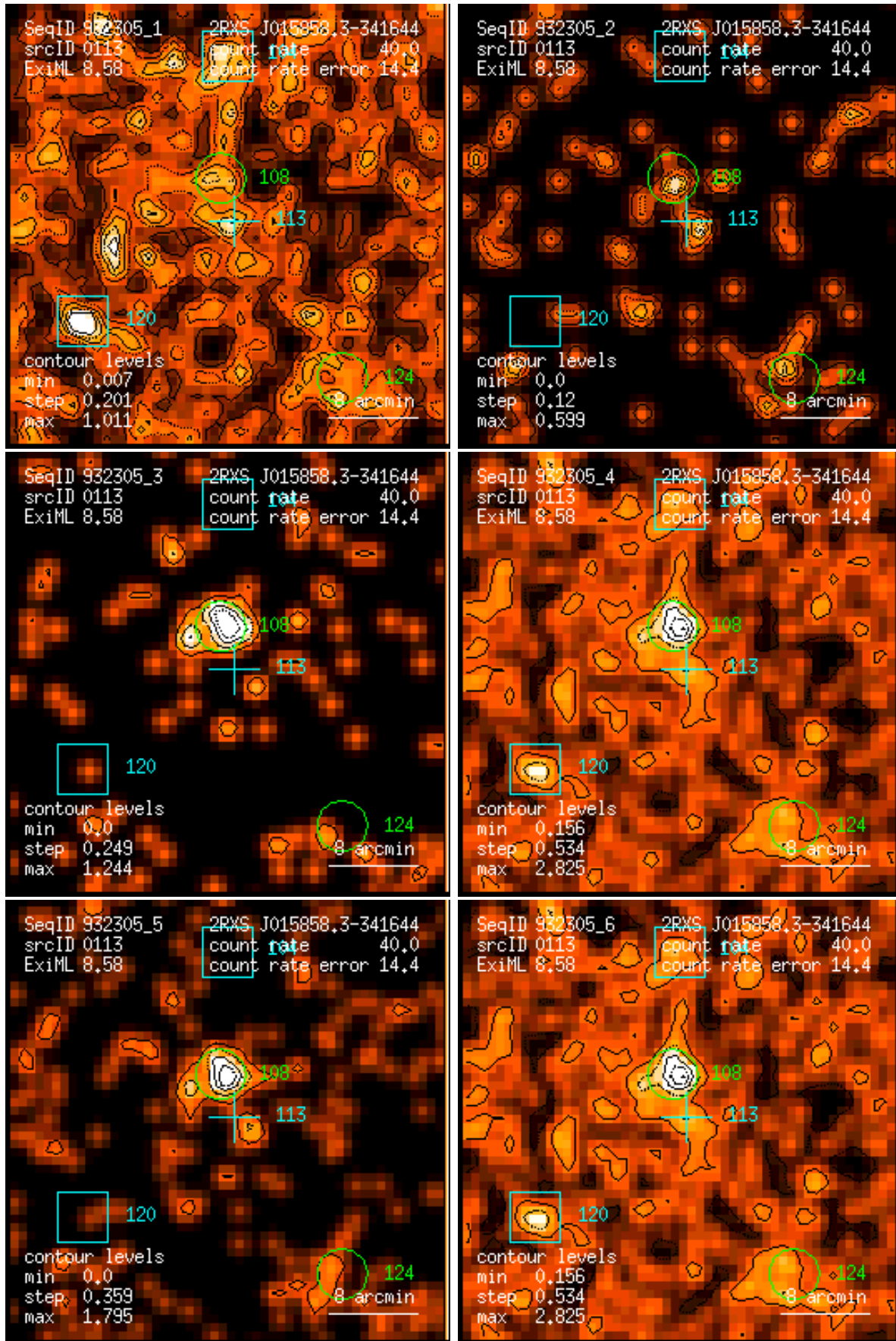
Figure 113: RASS 932305: detection 0113: band rate images, Gaussian filter: (1) PSPC channels 11 – 41, (2) 52 – 90, (3) 91 – 201, (4) 11 – 235, (5) 52 – 201, (6) 11 – 201. Broad band rates in counts/ks. Band rate contour levels in counts/ks/arcmin 2 .
