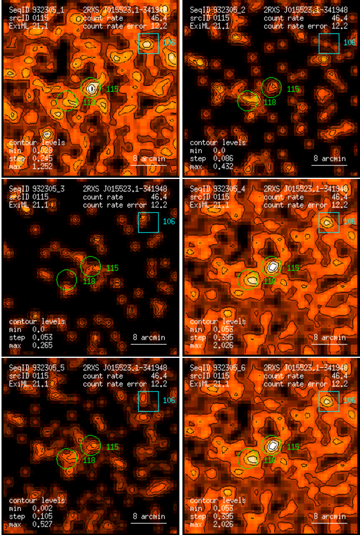
Figure 115: RASS 932305: detection 0115: band rate images, Gaussian filter: (1) PSPC channels 11 – 41, (2) 52 – 90, (3) 91 – 201, (4) 11 – 235, (5) 52 – 201, (6) 11 – 201. Broad band rates in counts/ks. Band rate contour levels in counts/ks/arcmin 2 .
