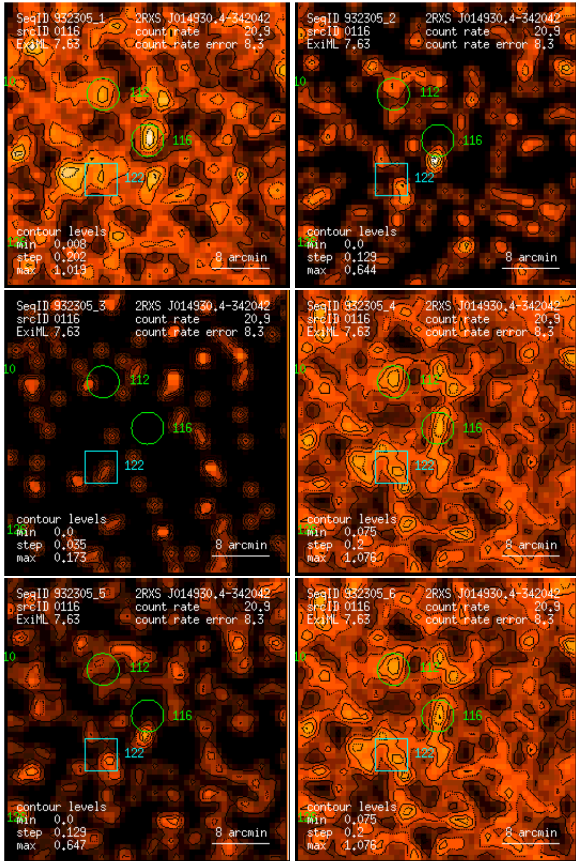
Figure 116: RASS 932305: detection 0116: band rate images, Gaussian filter: (1) PSPC channels 11 – 41, (2) 52 – 90, (3) 91 – 201, (4) 11 – 235, (5) 52 – 201, (6) 11 – 201. Broad band rates in counts/ks. Band rate contour levels in counts/ks/arcmin 2 .
