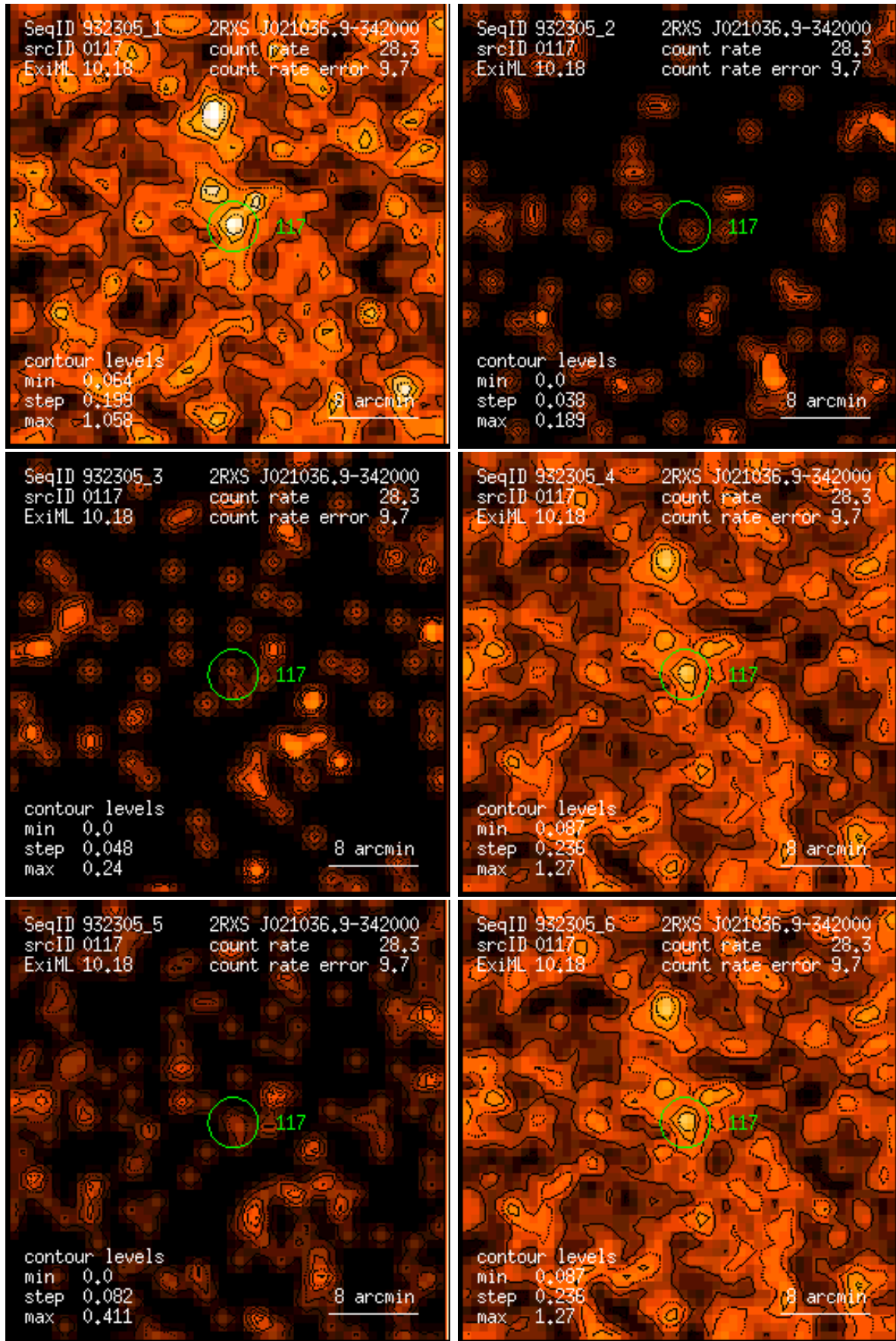
Figure 117: RASS 932305: detection 0117: band rate images, Gaussian filter: (1) PSPC channels 11 – 41, (2) 52 – 90, (3) 91 – 201, (4) 11 – 235, (5) 52 – 201, (6) 11 – 201. Broad band rates in counts/ks. Band rate contour levels in counts/ks/arcmin 2 .
