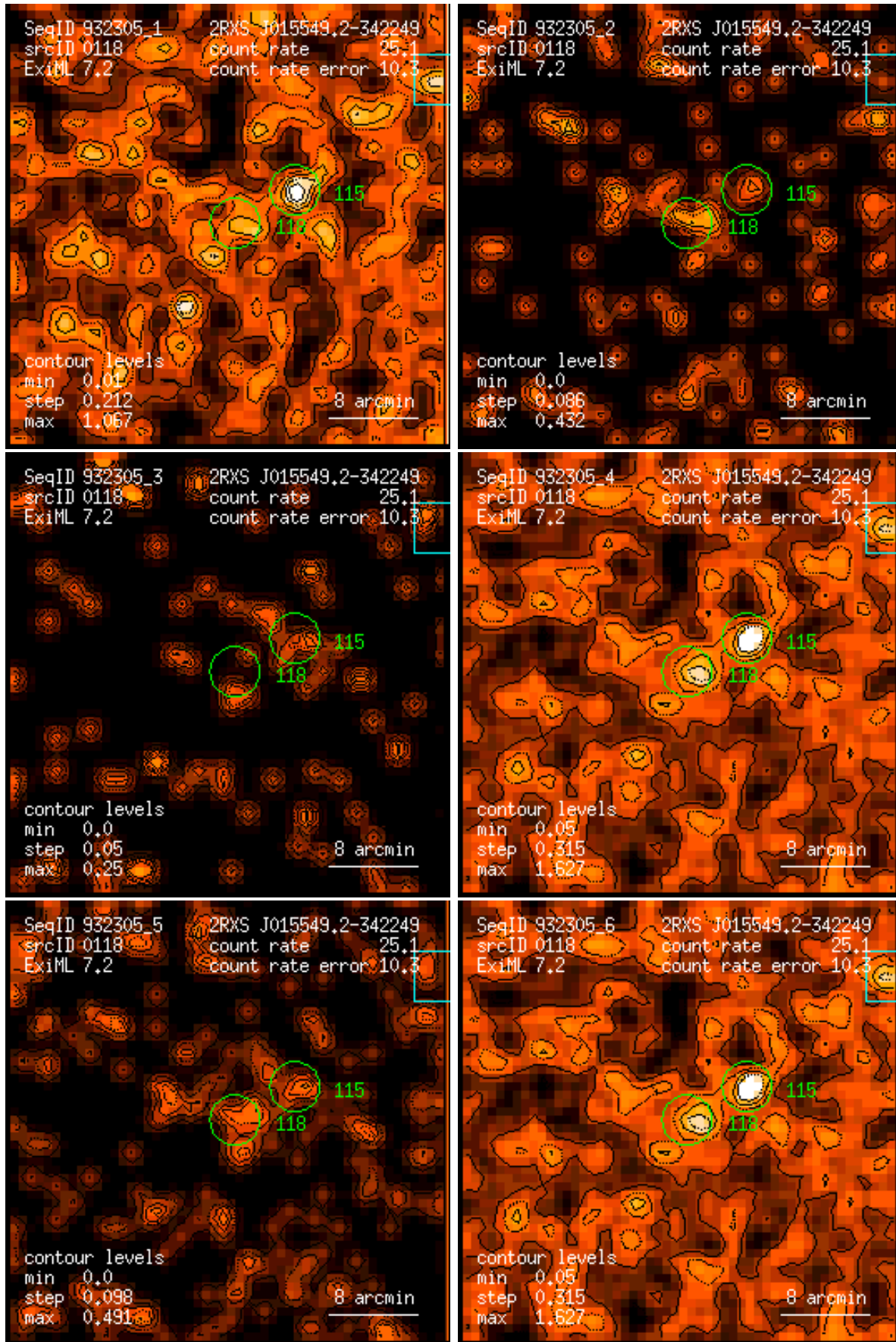
Figure 118: RASS 932305: detection 0118: band rate images, Gaussian filter: (1) PSPC channels 11 – 41, (2) 52 – 90, (3) 91 – 201, (4) 11 – 235, (5) 52 – 201, (6) 11 – 201. Broad band rates in counts/ks. Band rate contour levels in counts/ks/arcmin 2 .
