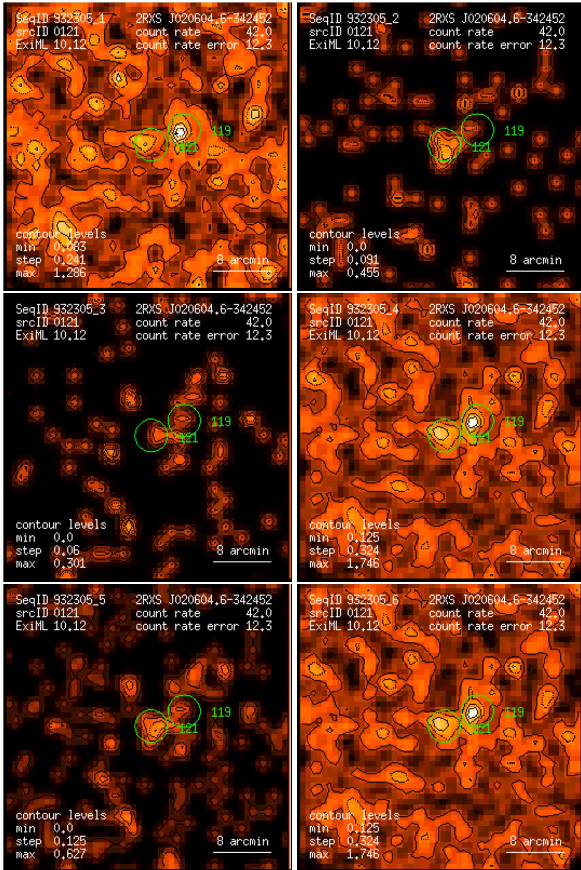
Figure 121: RASS 932305: detection 0121: band rate images, Gaussian filter: (1) PSPC channels 11 – 41, (2) 52 – 90, (3) 91 – 201, (4) 11 – 235, (5) 52 – 201, (6) 11 – 201. Broad band rates in counts/ks. Band rate contour levels in counts/ks/arcmin 2 .
