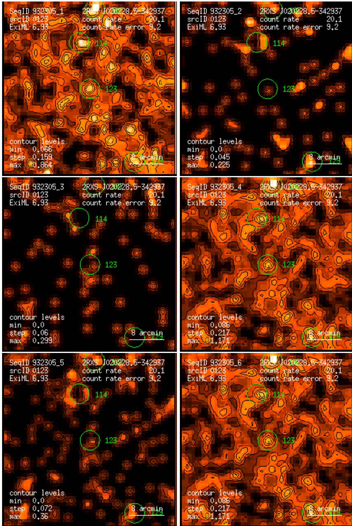
Figure 123: RASS 932305: detection 0123: band rate images, Gaussian filter: (1) PSPC channels 11 – 41, (2) 52 – 90, (3) 91 – 201, (4) 11 – 235, (5) 52 – 201, (6) 11 – 201. Broad band rates in counts/ks. Band rate contour levels in counts/ks/arcmin 2 .
