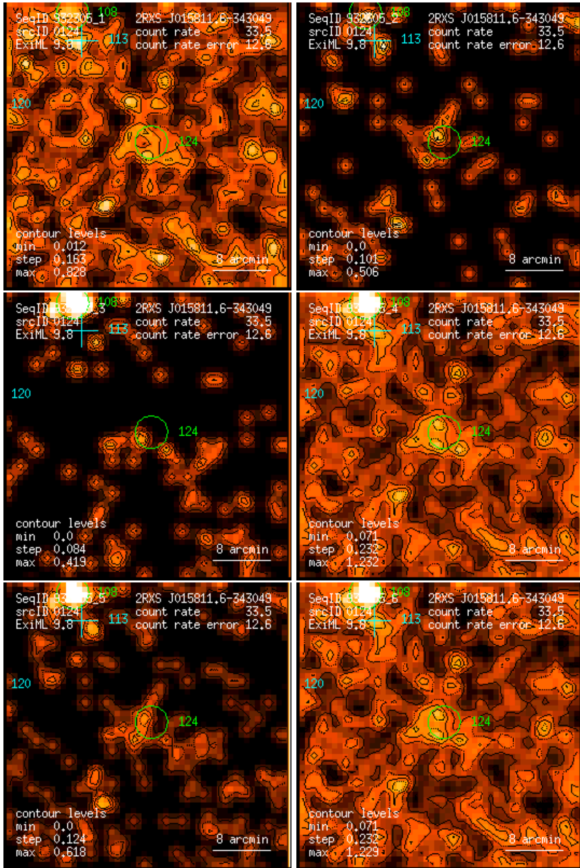
Figure 124: RASS 932305: detection 0124: band rate images, Gaussian filter: (1) PSPC channels 11 – 41, (2) 52 – 90, (3) 91 – 201, (4) 11 – 235, (5) 52 – 201, (6) 11 – 201. Broad band rates in counts/ks. Band rate contour levels in counts/ks/arcmin 2 .
