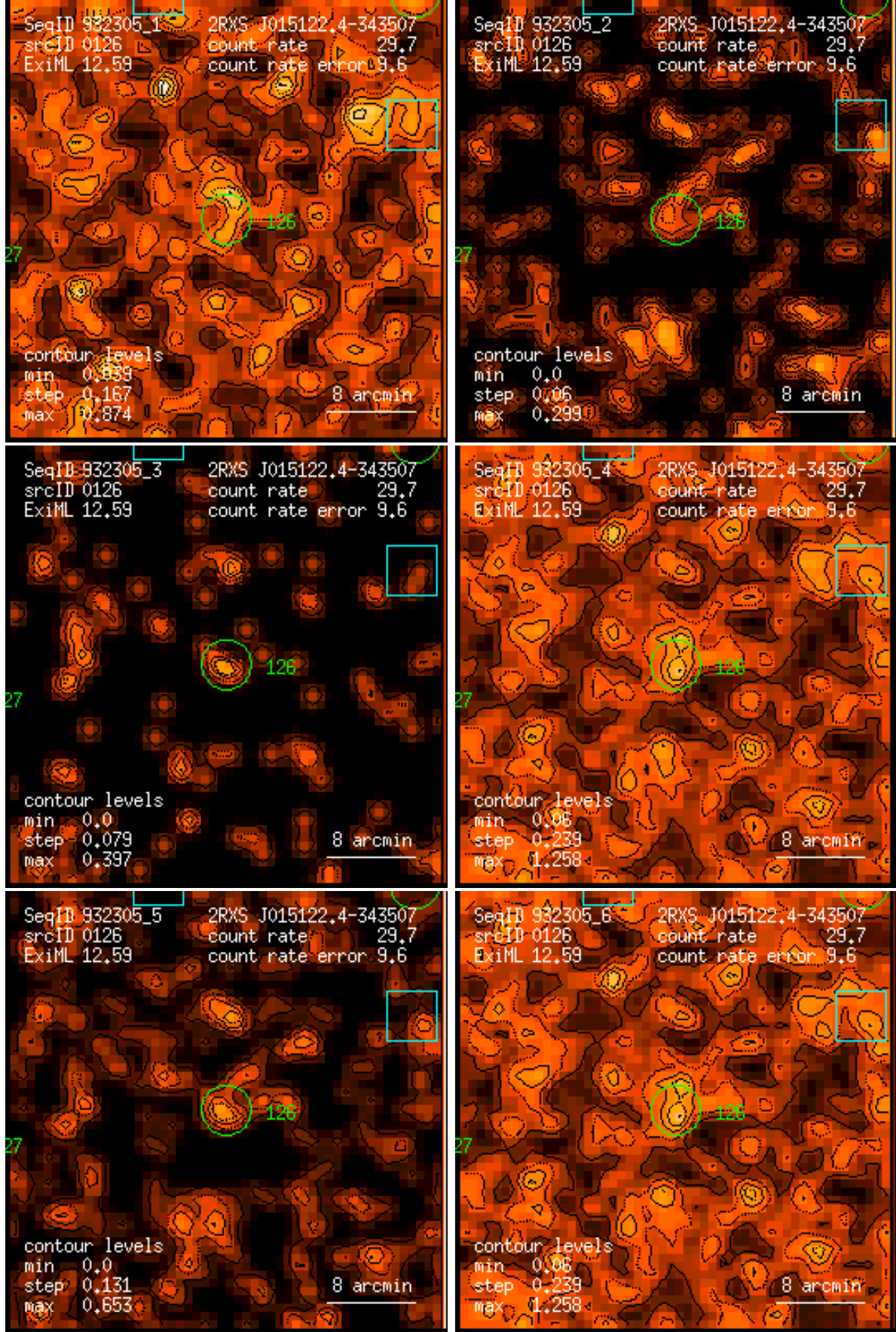
Figure 126: RASS 932305: detection 0126: band rate images, Gaussian filter: (1) PSPC channels 11 – 41, (2) 52 – 90, (3) 91 – 201, (4) 11 – 235, (5) 52 – 201, (6) 11 – 201. Broad band rates in counts/ks. Band rate contour levels in counts/ks/arcmin 2 .
