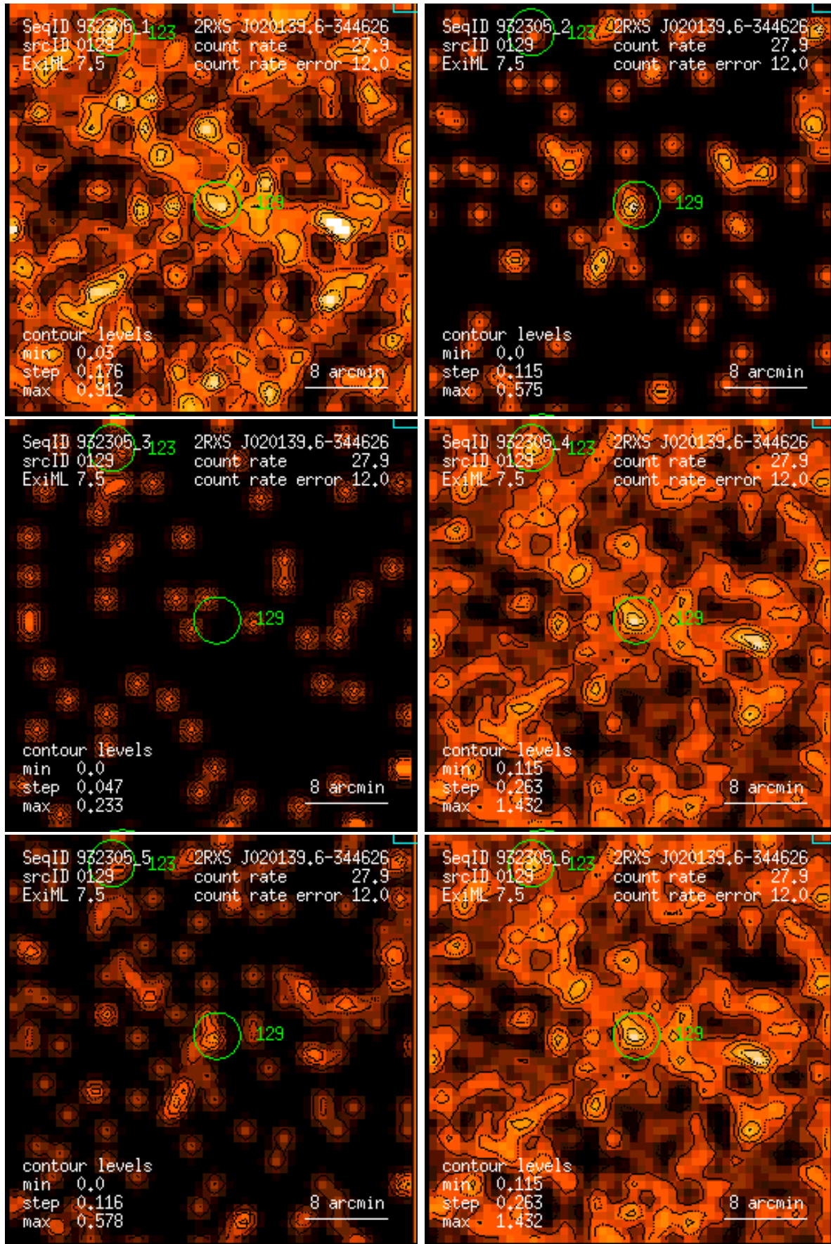
Figure 129: RASS 932305: detection 0129: band rate images, Gaussian filter: (1) PSPC channels 11 – 41, (2) 52 – 90, (3) 91 – 201, (4) 11 – 235, (5) 52 – 201, (6) 11 – 201. Broad band rates in counts/ks. Band rate contour levels in counts/ks/arcmin 2 .
