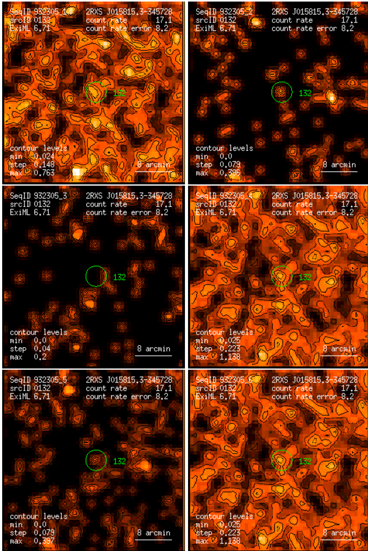
Figure 132: RASS 932305: detection 0132: band rate images, Gaussian filter: (1) PSPC channels 11 – 41, (2) 52 – 90, (3) 91 – 201, (4) 11 – 235, (5) 52 – 201, (6) 11 – 201. Broad band rates in counts/ks. Band rate contour levels in counts/ks/arcmin 2 .
