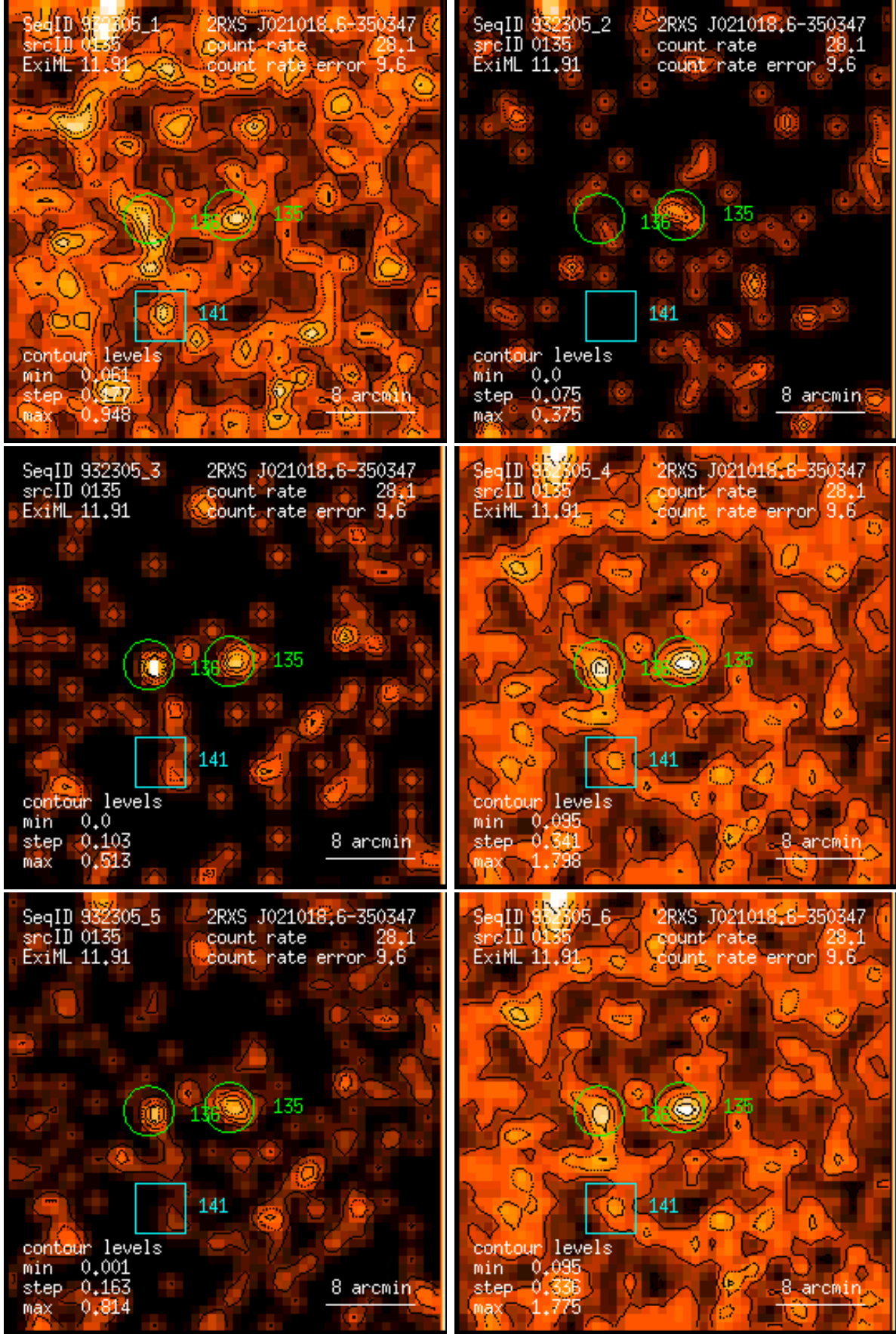
Figure 135: RASS 932305: detection 0135: band rate images, Gaussian filter: (1) PSPC channels 11 – 41, (2) 52 – 90, (3) 91 – 201, (4) 11 – 235, (5) 52 – 201, (6) 11 – 201. Broad band rates in counts/ks. Band rate contour levels in counts/ks/arcmin 2 .
