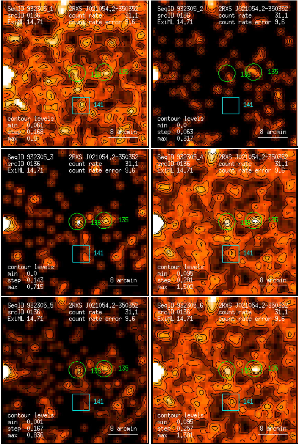
Figure 136: RASS 932305: detection 0136: band rate images, Gaussian filter: (1) PSPC channels 11 – 41, (2) 52 – 90, (3) 91 – 201, (4) 11 – 235, (5) 52 – 201, (6) 11 – 201. Broad band rates in counts/ks. Band rate contour levels in counts/ks/arcmin 2 .
