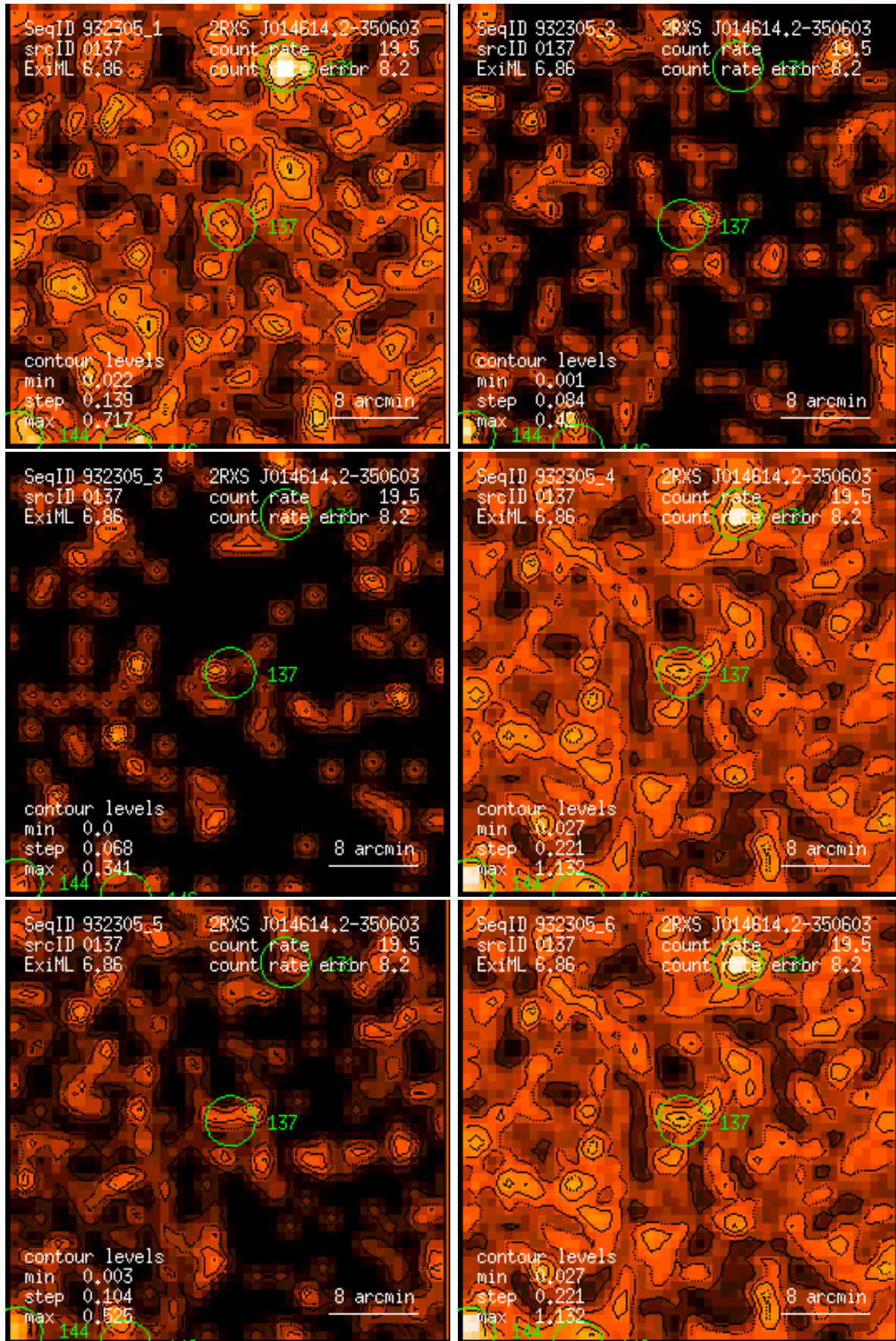
Figure 137: RASS 932305: detection 0137: band rate images, Gaussian filter: (1) PSPC channels 11 – 41, (2) 52 – 90, (3) 91 – 201, (4) 11 – 235, (5) 52 – 201, (6) 11 – 201. Broad band rates in counts/ks. Band rate contour levels in counts/ks/arcmin 2 .
