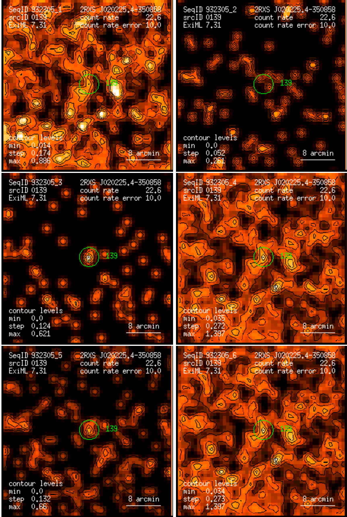
Figure 139: RASS 932305: detection 0139: band rate images, Gaussian filter: (1) PSPC channels 11 – 41, (2) 52 – 90, (3) 91 – 201, (4) 11 – 235, (5) 52 – 201, (6) 11 – 201. Broad band rates in counts/ks. Band rate contour levels in counts/ks/arcmin 2 .
