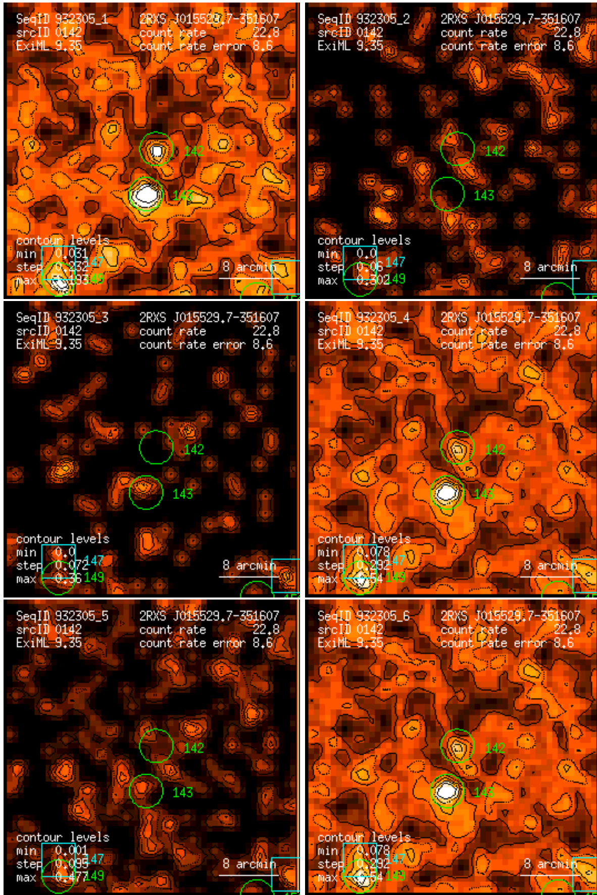
Figure 142: RASS 932305: detection 0142: band rate images, Gaussian filter: (1) PSPC channels 11 – 41, (2) 52 – 90, (3) 91 – 201, (4) 11 – 235, (5) 52 – 201, (6) 11 – 201. Broad band rates in counts/ks. Band rate contour levels in counts/ks/arcmin 2 .
