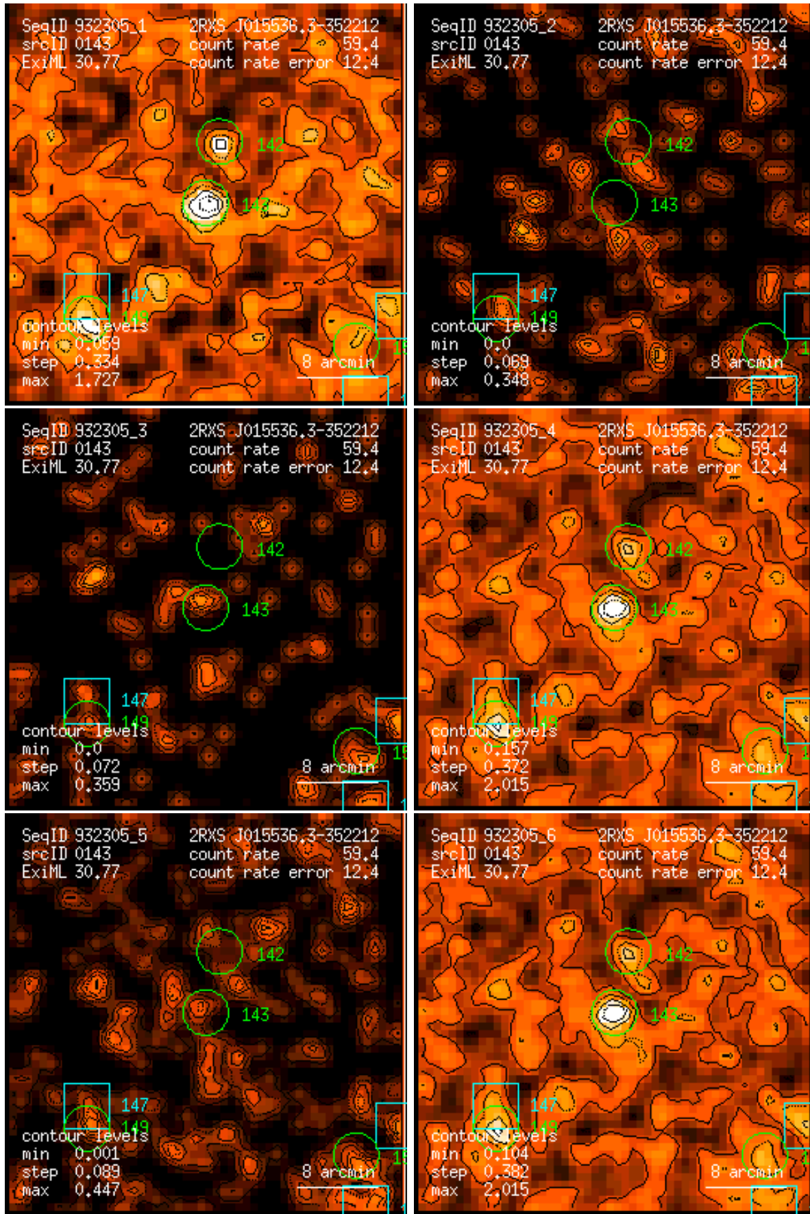
Figure 143: RASS 932305: detection 0143: band rate images, Gaussian filter: (1) PSPC channels 11 – 41, (2) 52 – 90, (3) 91 – 201, (4) 11 – 235, (5) 52 – 201, (6) 11 – 201. Broad band rates in counts/ks. Band rate contour levels in counts/ks/arcmin 2 .
