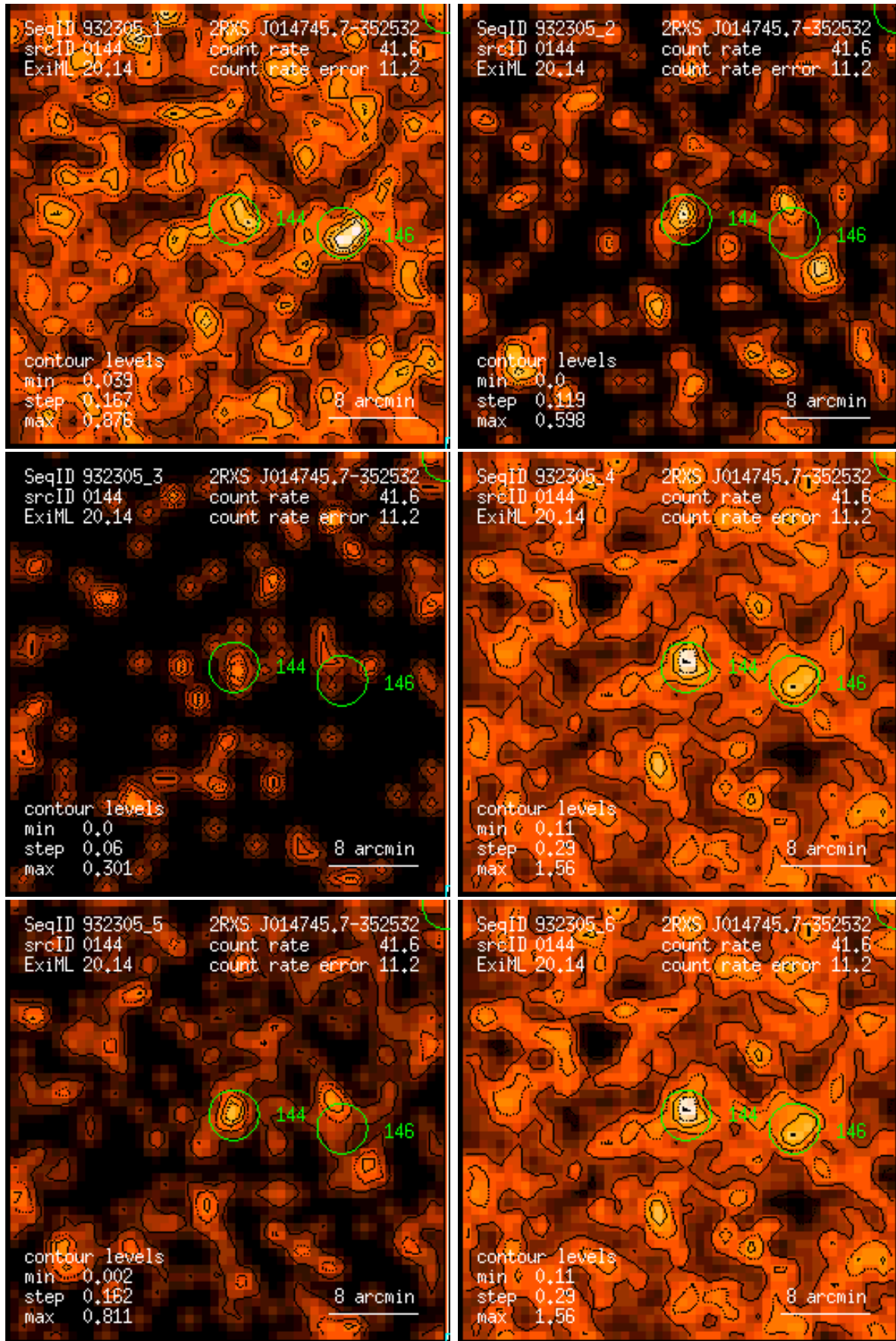
Figure 144: RASS 932305: detection 0144: band rate images, Gaussian filter: (1) PSPC channels 11 – 41, (2) 52 – 90, (3) 91 – 201, (4) 11 – 235, (5) 52 – 201, (6) 11 – 201. Broad band rates in counts/ks. Band rate contour levels in counts/ks/arcmin 2 .
