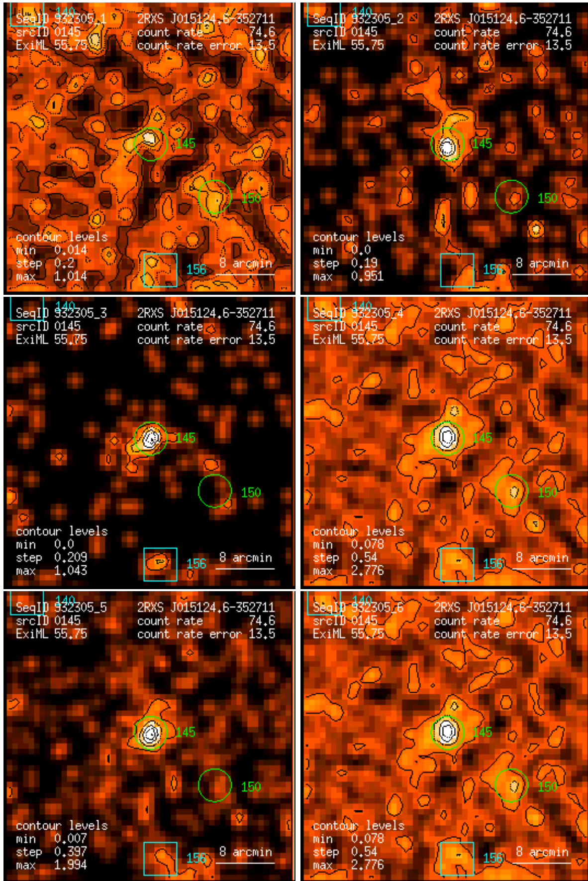
Figure 145: RASS 932305: detection 0145: band rate images, Gaussian filter: (1) PSPC channels 11 – 41, (2) 52 – 90, (3) 91 – 201, (4) 11 – 235, (5) 52 – 201, (6) 11 – 201. Broad band rates in counts/ks. Band rate contour levels in counts/ks/arcmin 2 .
