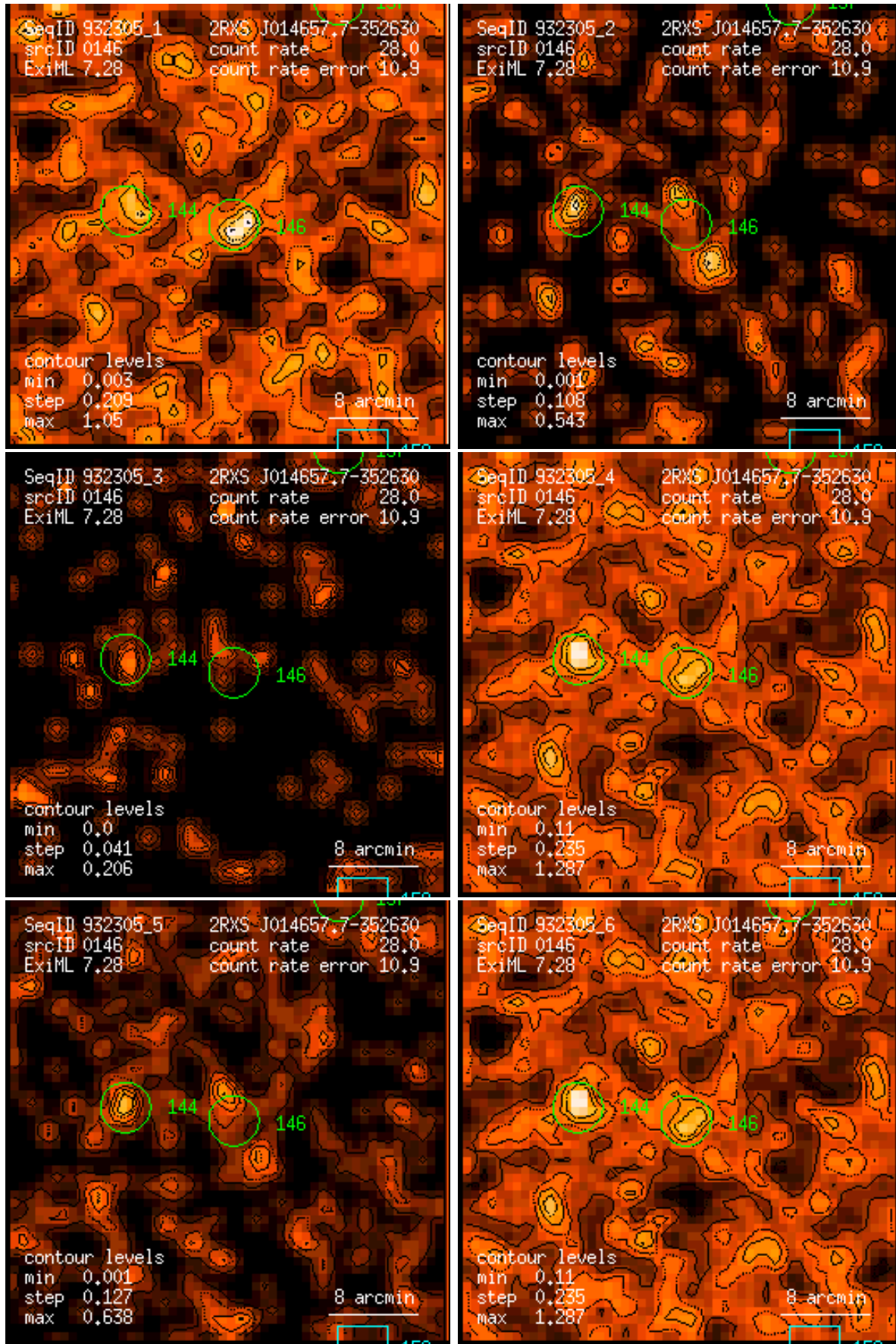
Figure 146: RASS 932305: detection 0146: band rate images, Gaussian filter: (1) PSPC channels 11 – 41, (2) 52 – 90, (3) 91 – 201, (4) 11 – 235, (5) 52 – 201, (6) 11 – 201. Broad band rates in counts/ks. Band rate contour levels in counts/ks/arcmin 2 .
