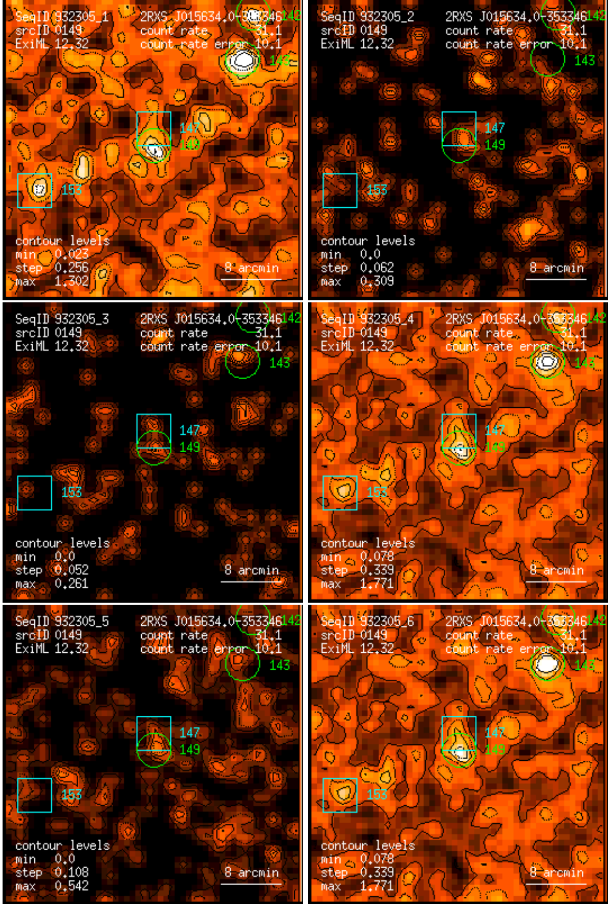
Figure 149: RASS 932305: detection 0149: band rate images, Gaussian filter: (1) PSPC channels 11 – 41, (2) 52 – 90, (3) 91 – 201, (4) 11 – 235, (5) 52 – 201, (6) 11 – 201. Broad band rates in counts/ks. Band rate contour levels in counts/ks/arcmin 2 .
