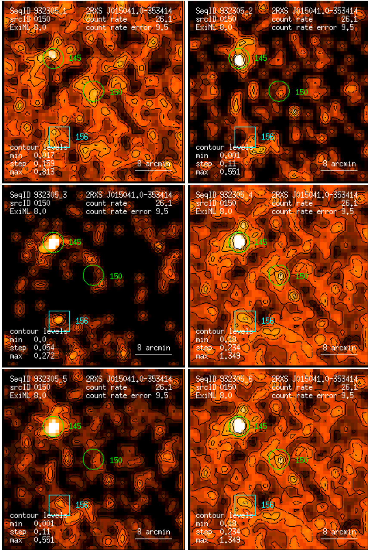
Figure 150: RASS 932305: detection 0150: band rate images, Gaussian filter: (1) PSPC channels 11 – 41, (2) 52 – 90, (3) 91 – 201, (4) 11 – 235, (5) 52 – 201, (6) 11 – 201. Broad band rates in counts/ks. Band rate contour levels in counts/ks/arcmin 2 .
