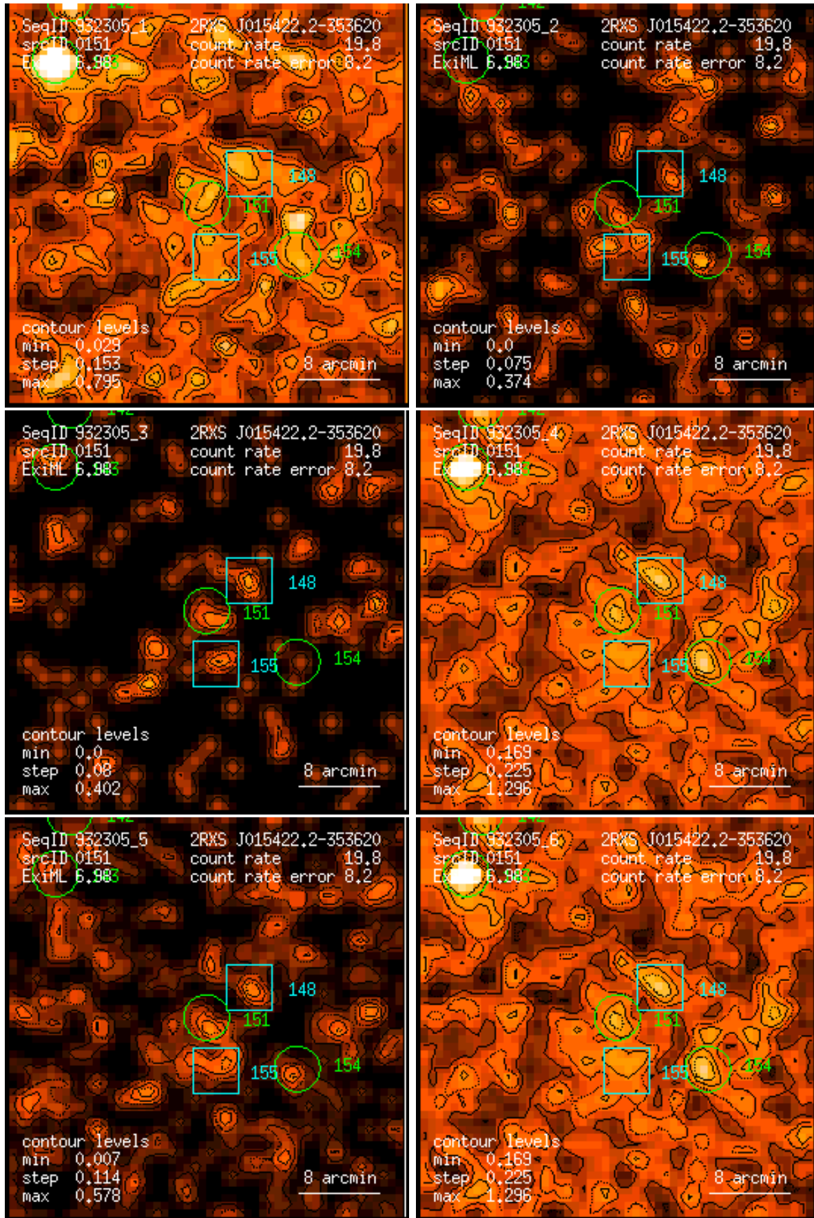
Figure 151: RASS 932305: detection 0151: band rate images, Gaussian filter: (1) PSPC channels 11 – 41, (2) 52 – 90, (3) 91 – 201, (4) 11 – 235, (5) 52 – 201, (6) 11 – 201. Broad band rates in counts/ks. Band rate contour levels in counts/ks/arcmin 2 .
