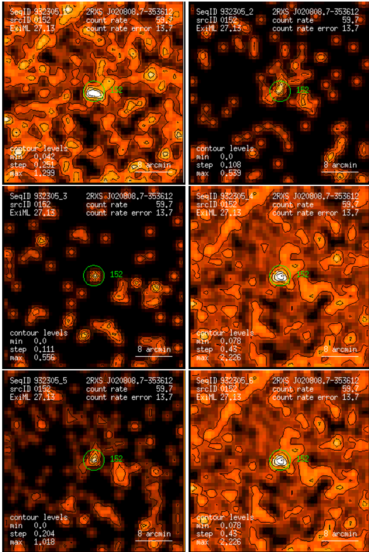
Figure 152: RASS 932305: detection 0152: band rate images, Gaussian filter: (1) PSPC channels 11 – 41, (2) 52 – 90, (3) 91 – 201, (4) 11 – 235, (5) 52 – 201, (6) 11 – 201. Broad band rates in counts/ks. Band rate contour levels in counts/ks/arcmin 2 .
