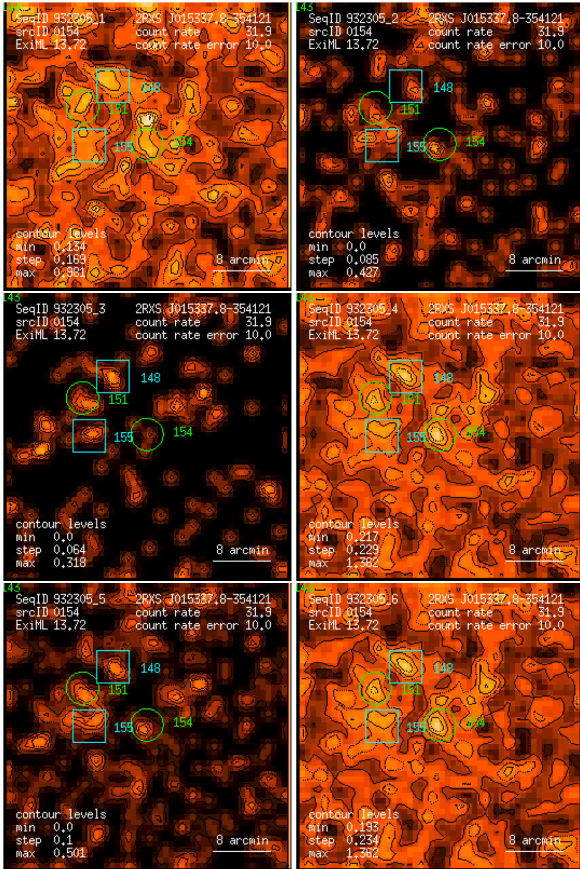
Figure 154: RASS 932305: detection 0154: band rate images, Gaussian filter: (1) PSPC channels 11 – 41, (2) 52 – 90, (3) 91 – 201, (4) 11 – 235, (5) 52 – 201, (6) 11 – 201. Broad band rates in counts/ks. Band rate contour levels in counts/ks/arcmin 2 .
