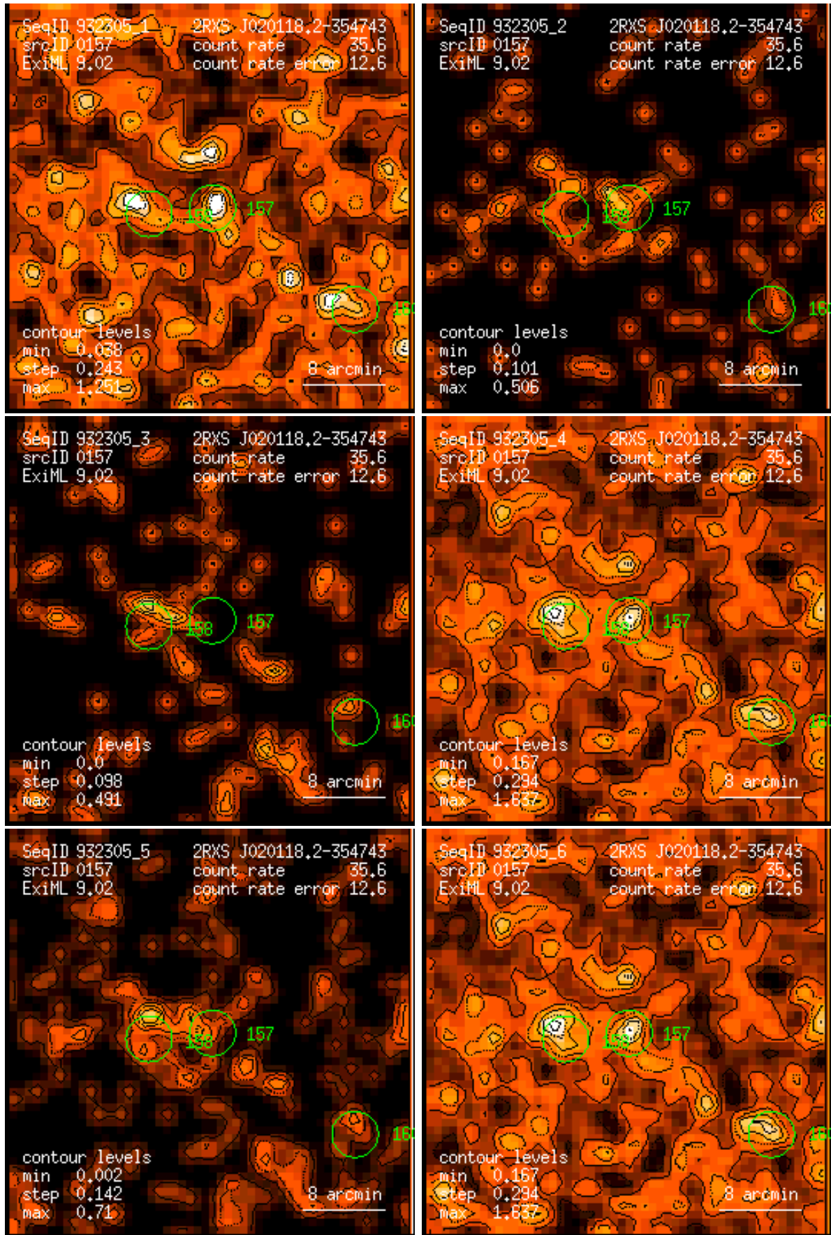
Figure 157: RASS 932305: detection 0157: band rate images, Gaussian filter: (1) PSPC channels 11 – 41, (2) 52 – 90, (3) 91 – 201, (4) 11 – 235, (5) 52 – 201, (6) 11 – 201. Broad band rates in counts/ks. Band rate contour levels in counts/ks/arcmin 2 .
