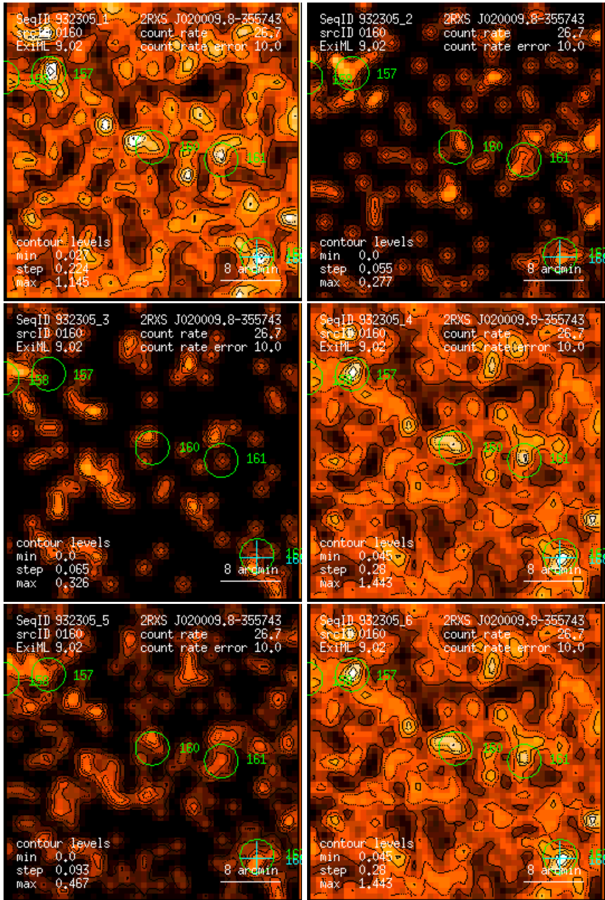
Figure 160: RASS 932305: detection 0160: band rate images, Gaussian filter: (1) PSPC channels 11 – 41, (2) 52 – 90, (3) 91 – 201, (4) 11 – 235, (5) 52 – 201, (6) 11 – 201. Broad band rates in counts/ks. Band rate contour levels in counts/ks/arcmin 2 .
