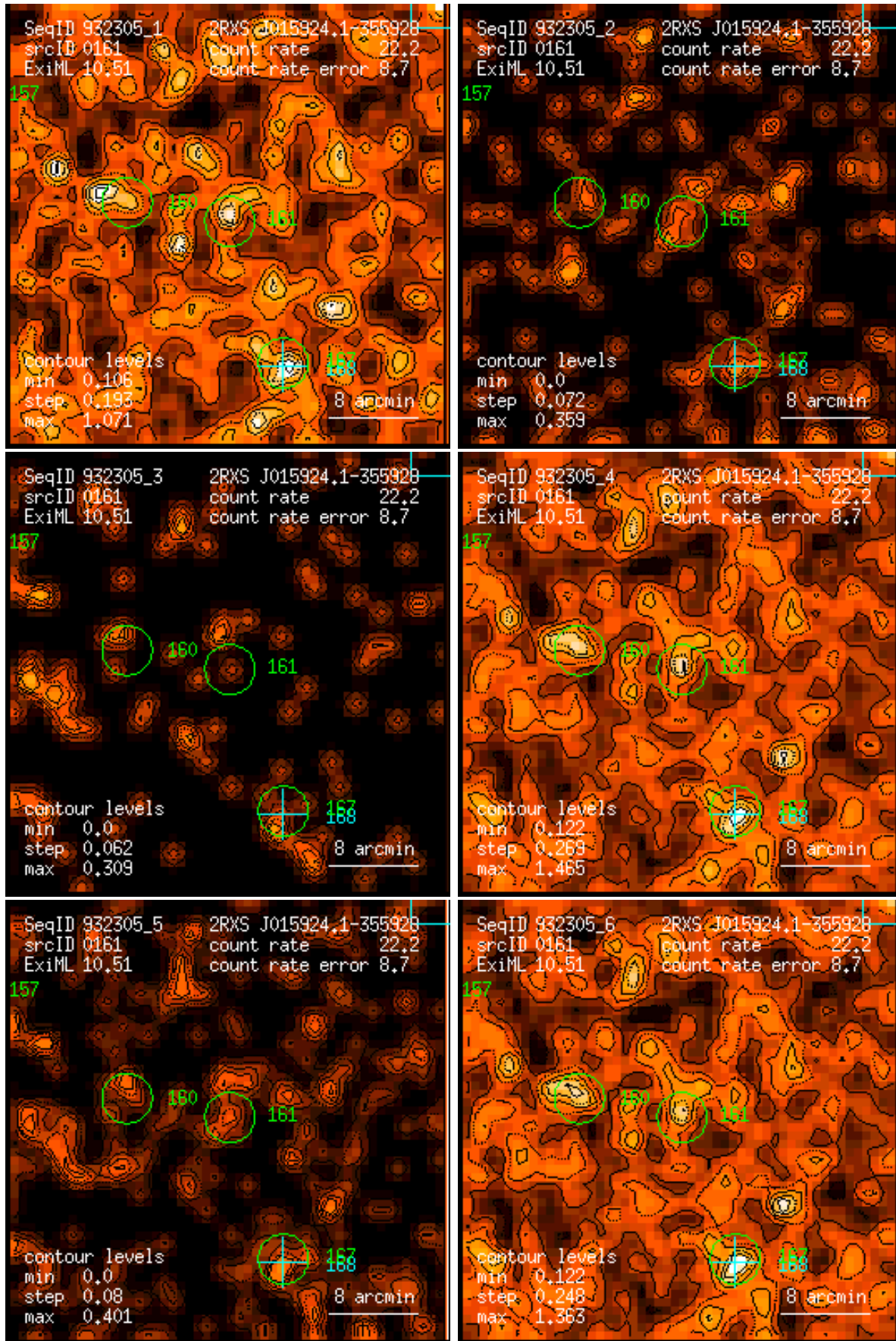
Figure 161: RASS 932305: detection 0161: band rate images, Gaussian filter: (1) PSPC channels 11 – 41, (2) 52 – 90, (3) 91 – 201, (4) 11 – 235, (5) 52 – 201, (6) 11 – 201. Broad band rates in counts/ks. Band rate contour levels in counts/ks/arcmin 2 .
