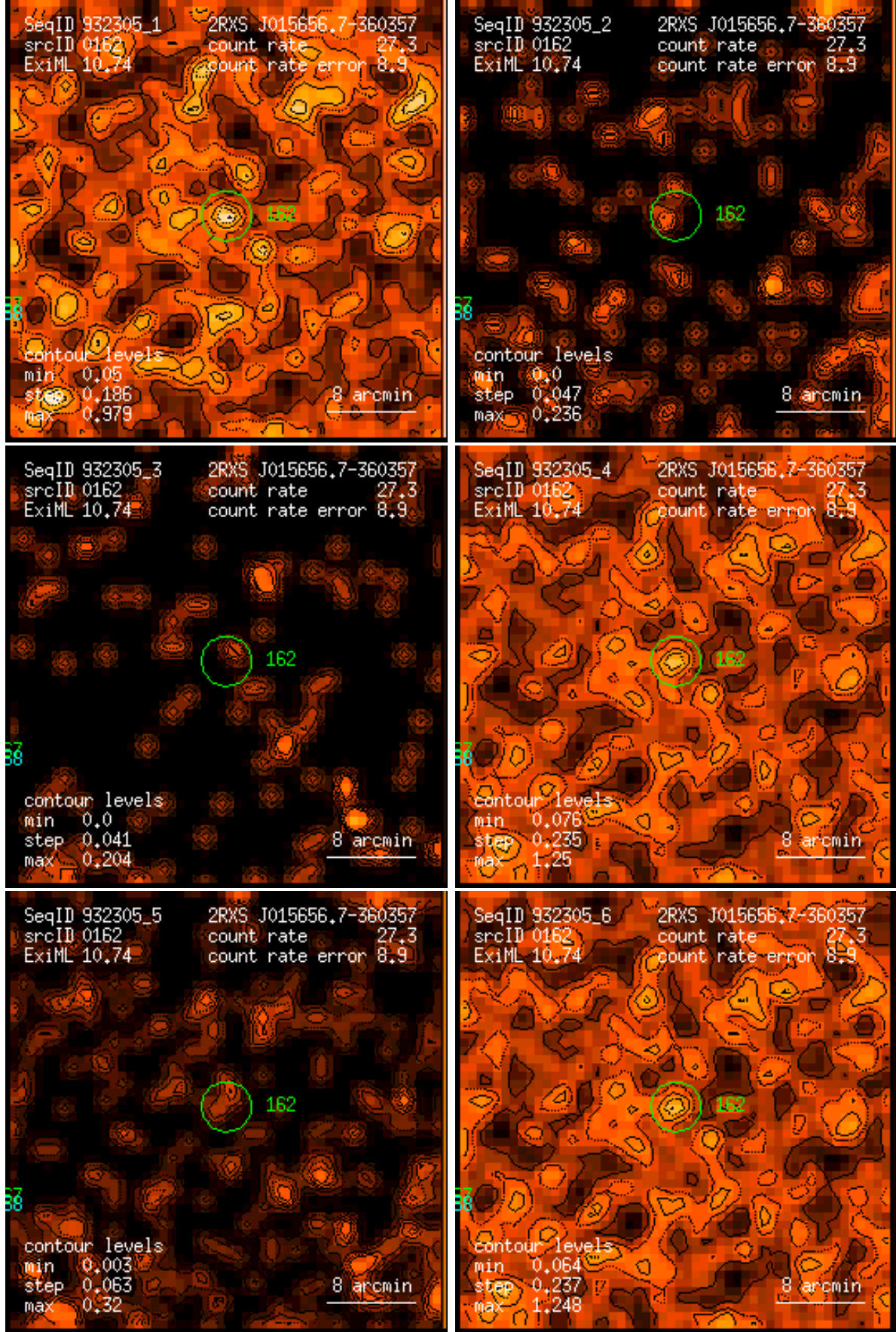
Figure 162: RASS 932305: detection 0162: band rate images, Gaussian filter: (1) PSPC channels 11 – 41, (2) 52 – 90, (3) 91 – 201, (4) 11 – 235, (5) 52 – 201, (6) 11 – 201. Broad band rates in counts/ks. Band rate contour levels in counts/ks/arcmin 2 .
