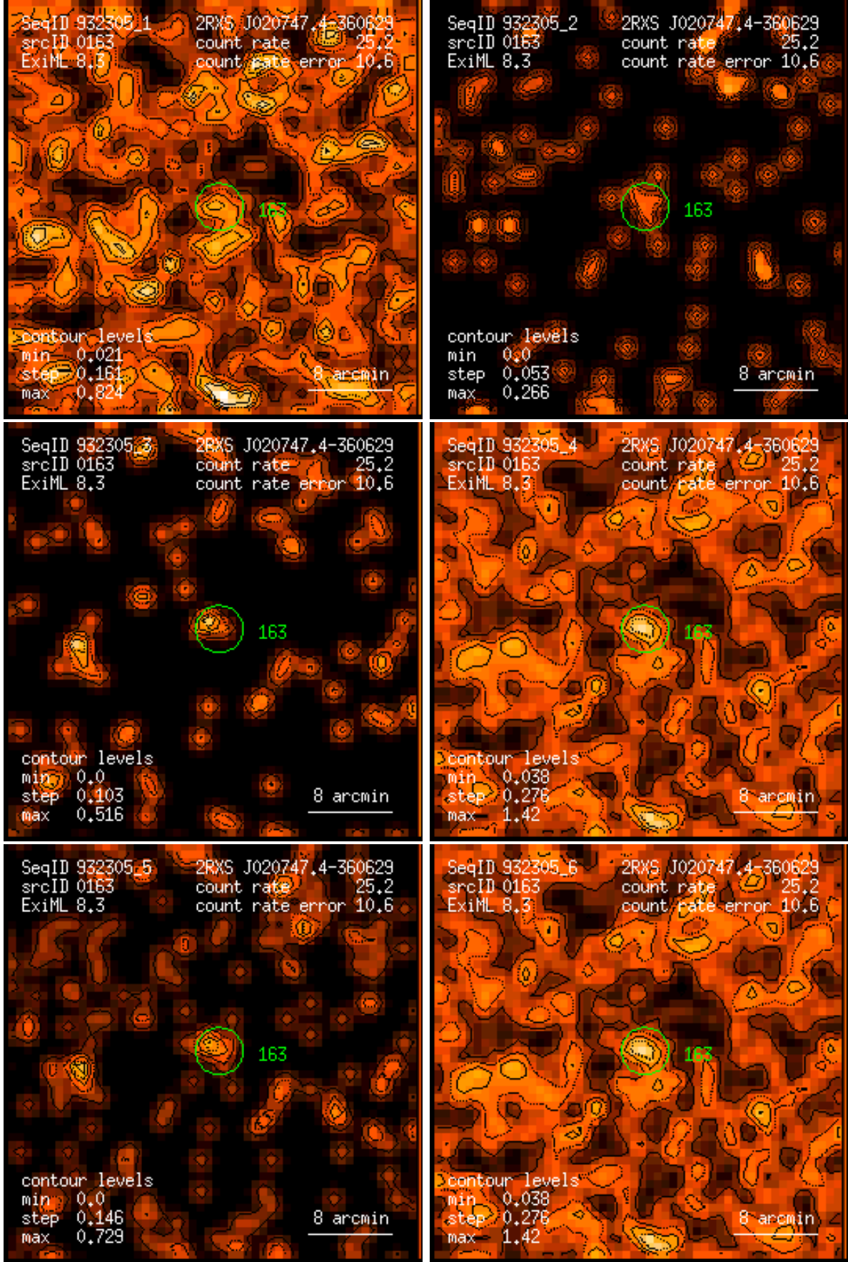
Figure 163: RASS 932305: detection 0163: band rate images, Gaussian filter: (1) PSPC channels 11 – 41, (2) 52 – 90, (3) 91 – 201, (4) 11 – 235, (5) 52 – 201, (6) 11 – 201. Broad band rates in counts/ks. Band rate contour levels in counts/ks/arcmin 2 .
