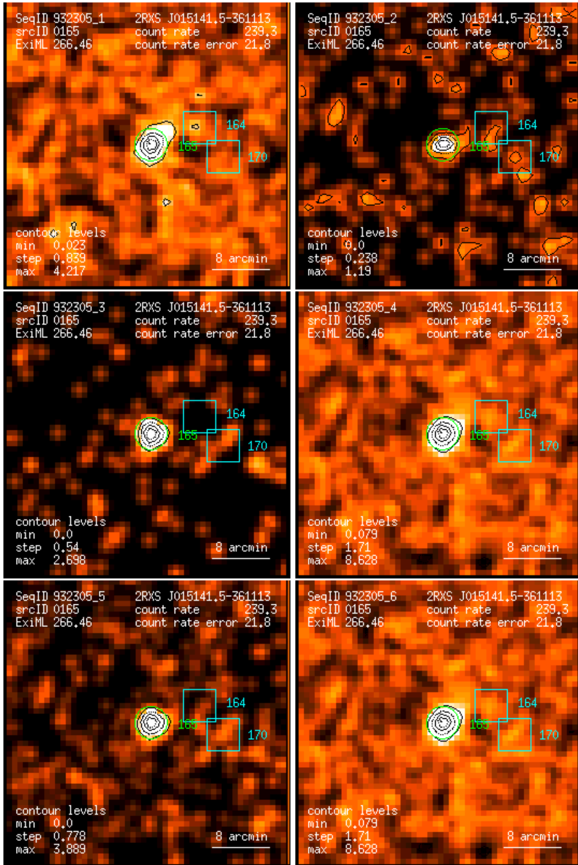
Figure 165: RASS 932305: detection 0165: band rate images, Gaussian filter: (1) PSPC channels 11 – 41, (2) 52 – 90, (3) 91 – 201, (4) 11 – 235, (5) 52 – 201, (6) 11 – 201. Broad band rates in counts/ks. Band rate contour levels in counts/ks/arcmin 2 .
