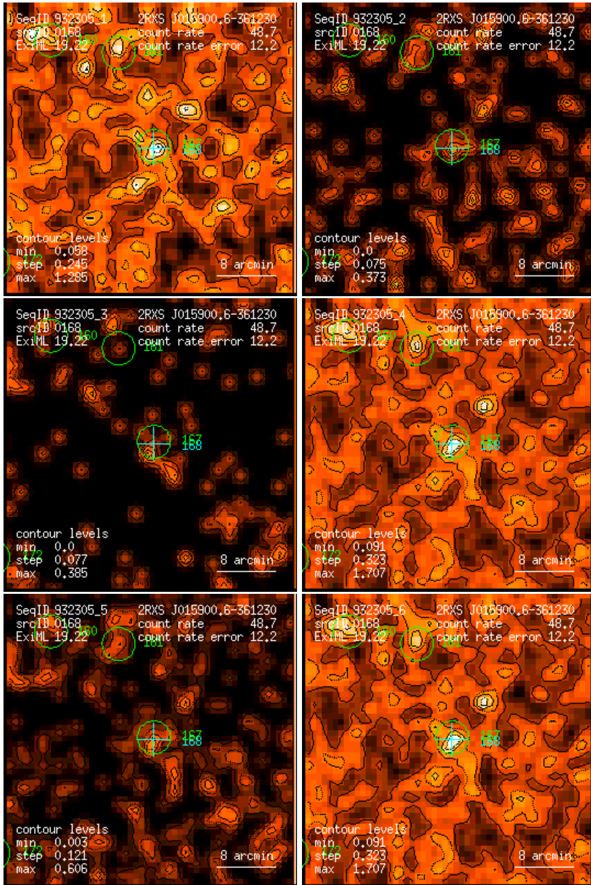
Figure 168: RASS 932305: detection 0168: band rate images, Gaussian filter: (1) PSPC channels 11 – 41, (2) 52 – 90, (3) 91 – 201, (4) 11 – 235, (5) 52 – 201, (6) 11 – 201. Broad band rates in counts/ks. Band rate contour levels in counts/ks/arcmin 2 .
