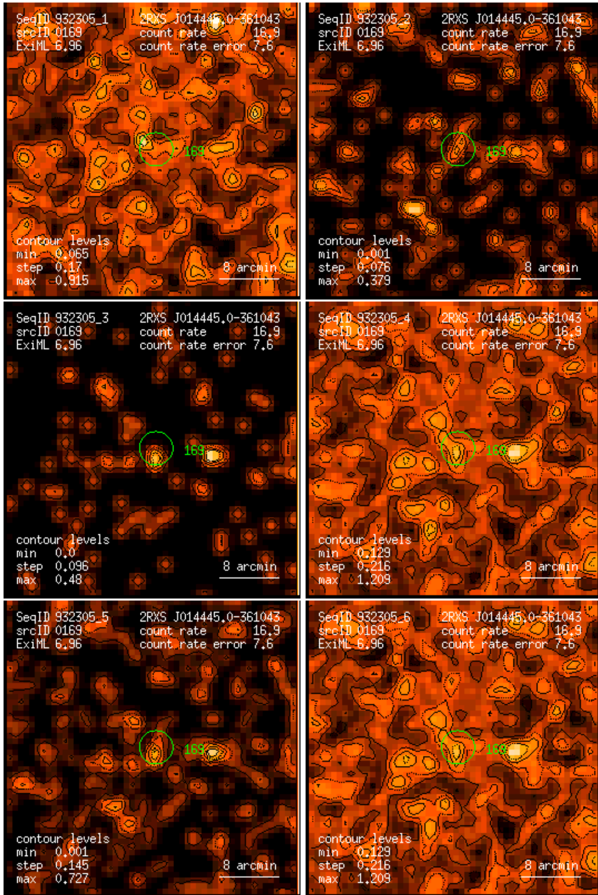
Figure 169: RASS 932305: detection 0169: band rate images, Gaussian filter: (1) PSPC channels 11 – 41, (2) 52 – 90, (3) 91 – 201, (4) 11 – 235, (5) 52 – 201, (6) 11 – 201. Broad band rates in counts/ks. Band rate contour levels in counts/ks/arcmin 2 .
