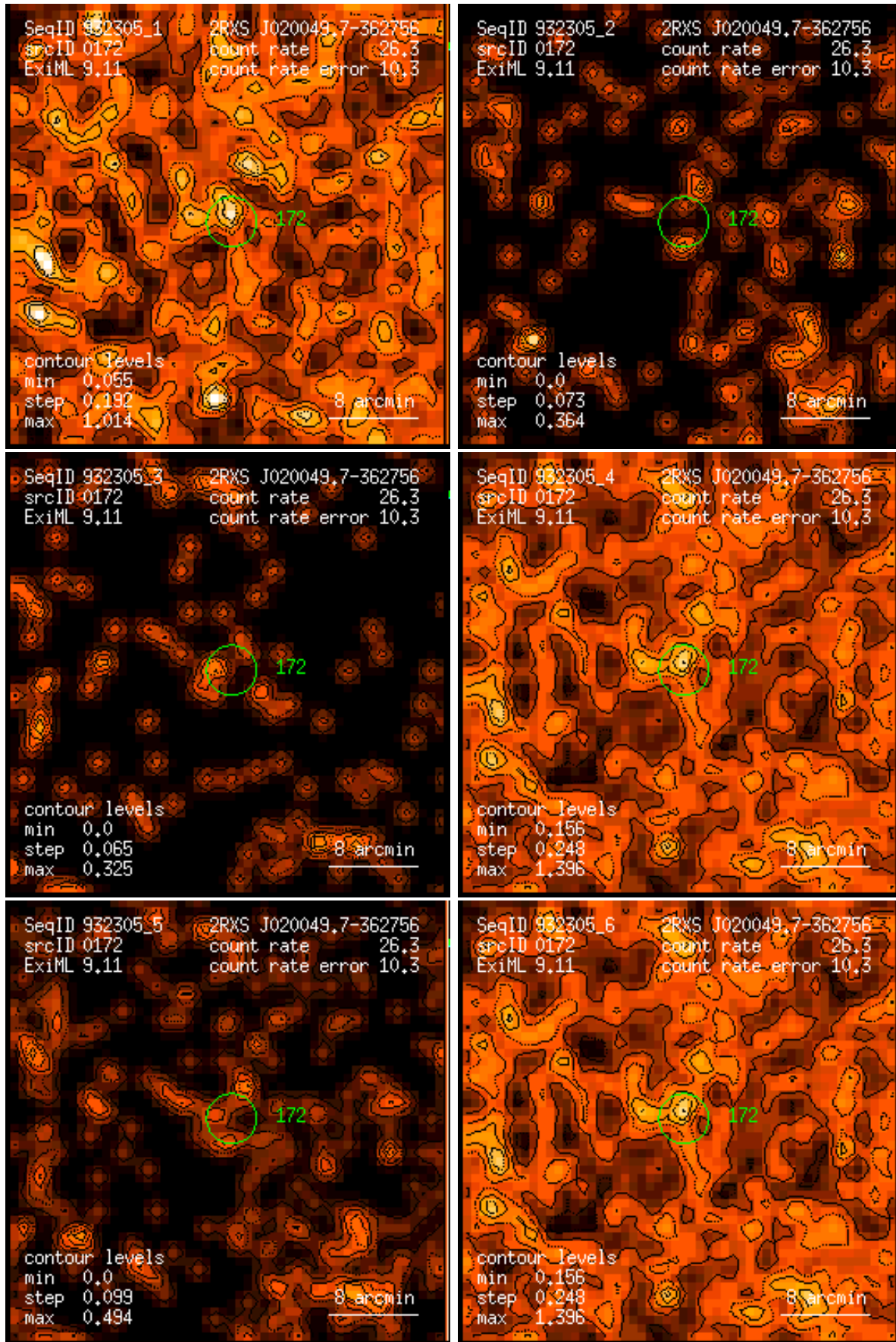
Figure 172: RASS 932305: detection 0172: band rate images, Gaussian filter: (1) PSPC channels 11 – 41, (2) 52 – 90, (3) 91 – 201, (4) 11 – 235, (5) 52 – 201, (6) 11 – 201. Broad band rates in counts/ks. Band rate contour levels in counts/ks/arcmin 2 .
