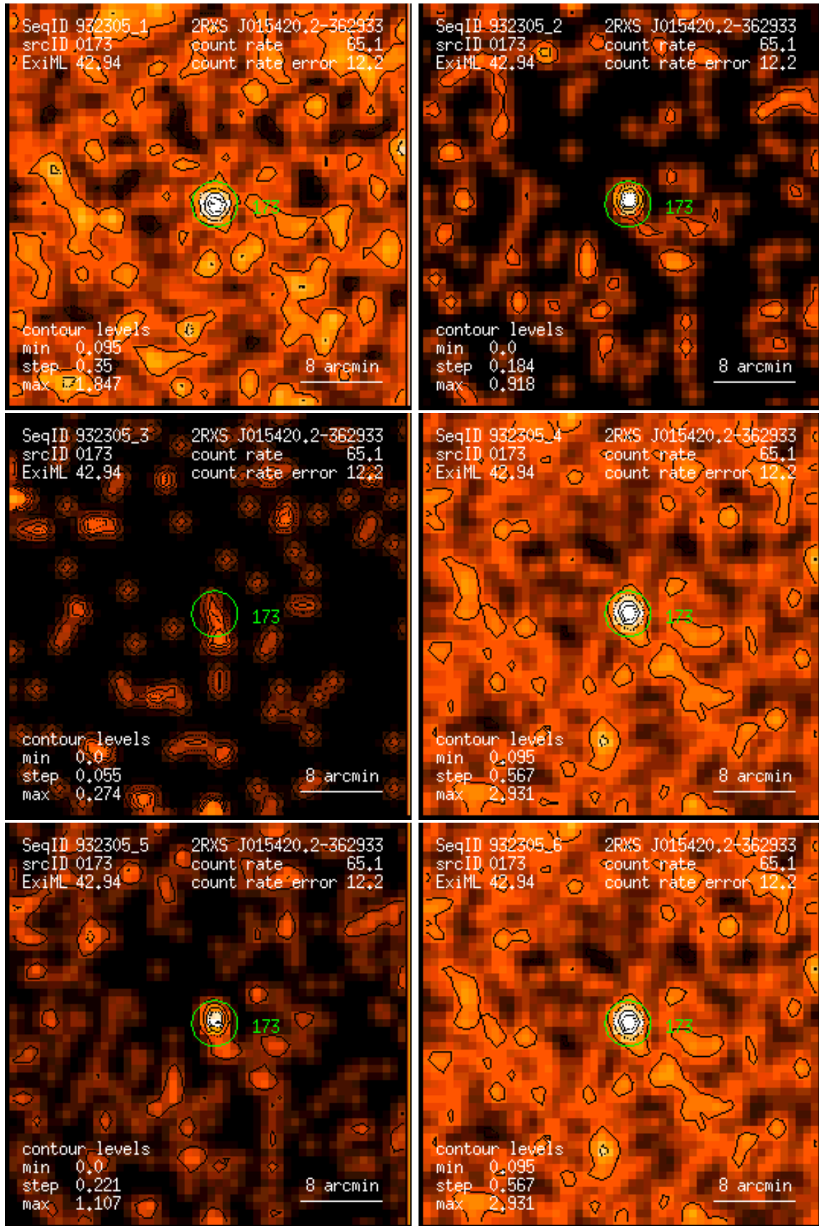
Figure 173: RASS 932305: detection 0173: band rate images, Gaussian filter: (1) PSPC channels 11 – 41, (2) 52 – 90, (3) 91 – 201, (4) 11 – 235, (5) 52 – 201, (6) 11 – 201. Broad band rates in counts/ks. Band rate contour levels in counts/ks/arcmin 2 .
