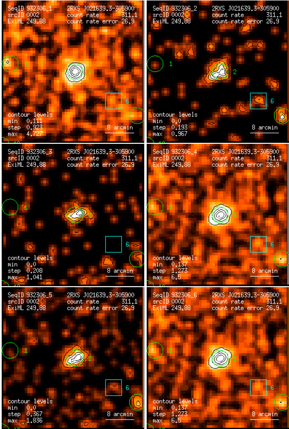
Figure 2: RASS 932306: detection 0002: band rate images, Gaussian filter: (1) PSPC channels 11 – 41, (2) 52 – 90, (3) 91 – 201, (4) 11 – 235, (5) 52 – 201, (6) 11 – 201. Broad band rates in counts/ks. Band rate contour levels in counts/ks/arcmin 2 .
