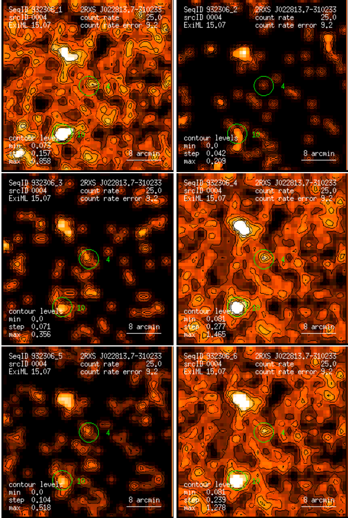
Figure 4: RASS 932306: detection 0004: band rate images, Gaussian filter: (1) PSPC channels 11 – 41, (2) 52 – 90, (3) 91 – 201, (4) 11 – 235, (5) 52 – 201, (6) 11 – 201. Broad band rates in counts/ks. Band rate contour levels in counts/ks/arcmin 2 .
