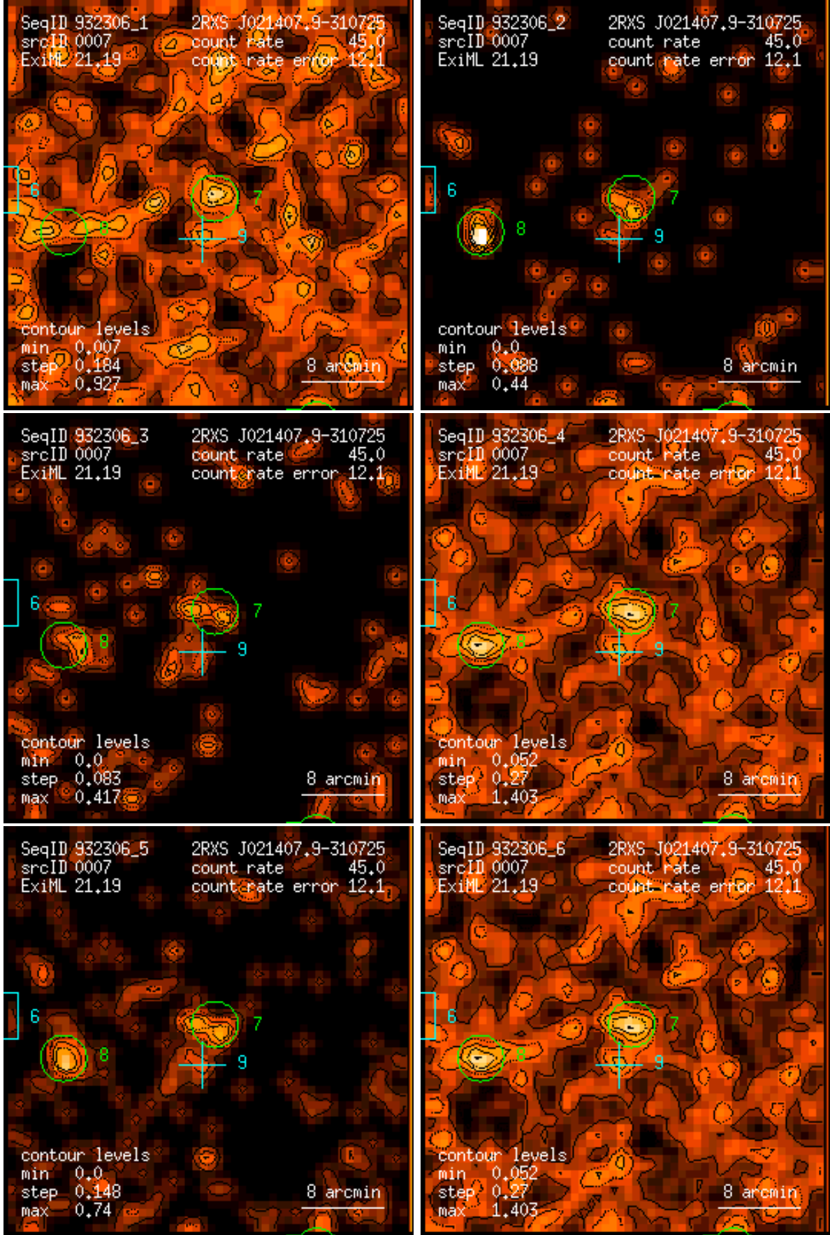
Figure 7: RASS 932306: detection 0007: band rate images, Gaussian filter: (1) PSPC channels 11 – 41, (2) 52 – 90, (3) 91 – 201, (4) 11 – 235, (5) 52 – 201, (6) 11 – 201. Broad band rates in counts/ks. Band rate contour levels in counts/ks/arcmin 2 .
