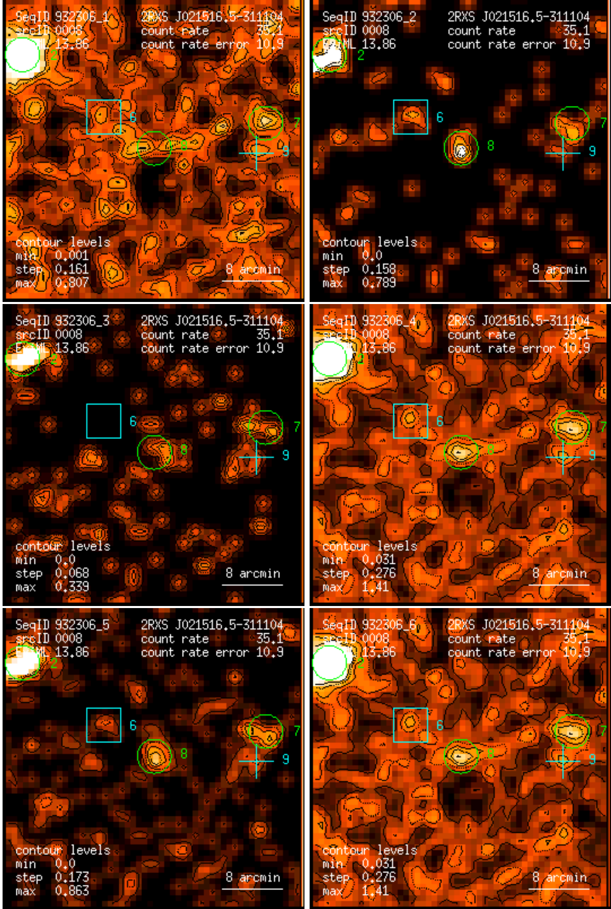
Figure 8: RASS 932306: detection 0008: band rate images, Gaussian filter: (1) PSPC channels 11 – 41, (2) 52 – 90, (3) 91 – 201, (4) 11 – 235, (5) 52 – 201, (6) 11 – 201. Broad band rates in counts/ks. Band rate contour levels in counts/ks/arcmin 2 .
