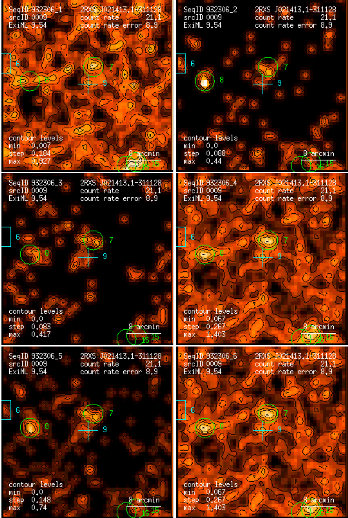
Figure 9: RASS 932306: detection 0009: band rate images, Gaussian filter: (1) PSPC channels 11 – 41, (2) 52 – 90, (3) 91 – 201, (4) 11 – 235, (5) 52 – 201, (6) 11 – 201. Broad band rates in counts/ks. Band rate contour levels in counts/ks/arcmin 2 .
