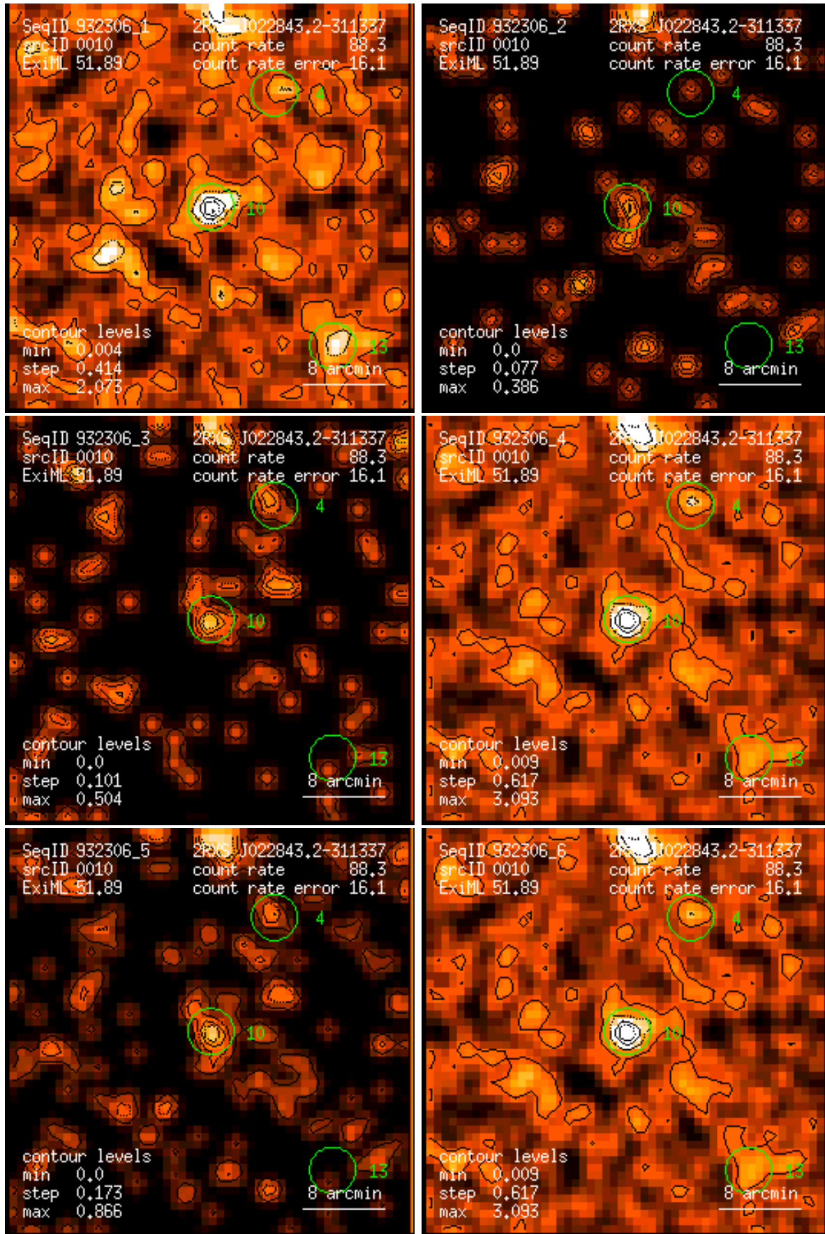
Figure 10: RASS 932306: detection 0010: band rate images, Gaussian filter: (1) PSPC channels 11 – 41, (2) 52 – 90, (3) 91 – 201, (4) 11 – 235, (5) 52 – 201, (6) 11 – 201. Broad band rates in counts/ks. Band rate contour levels in counts/ks/arcmin 2 .
