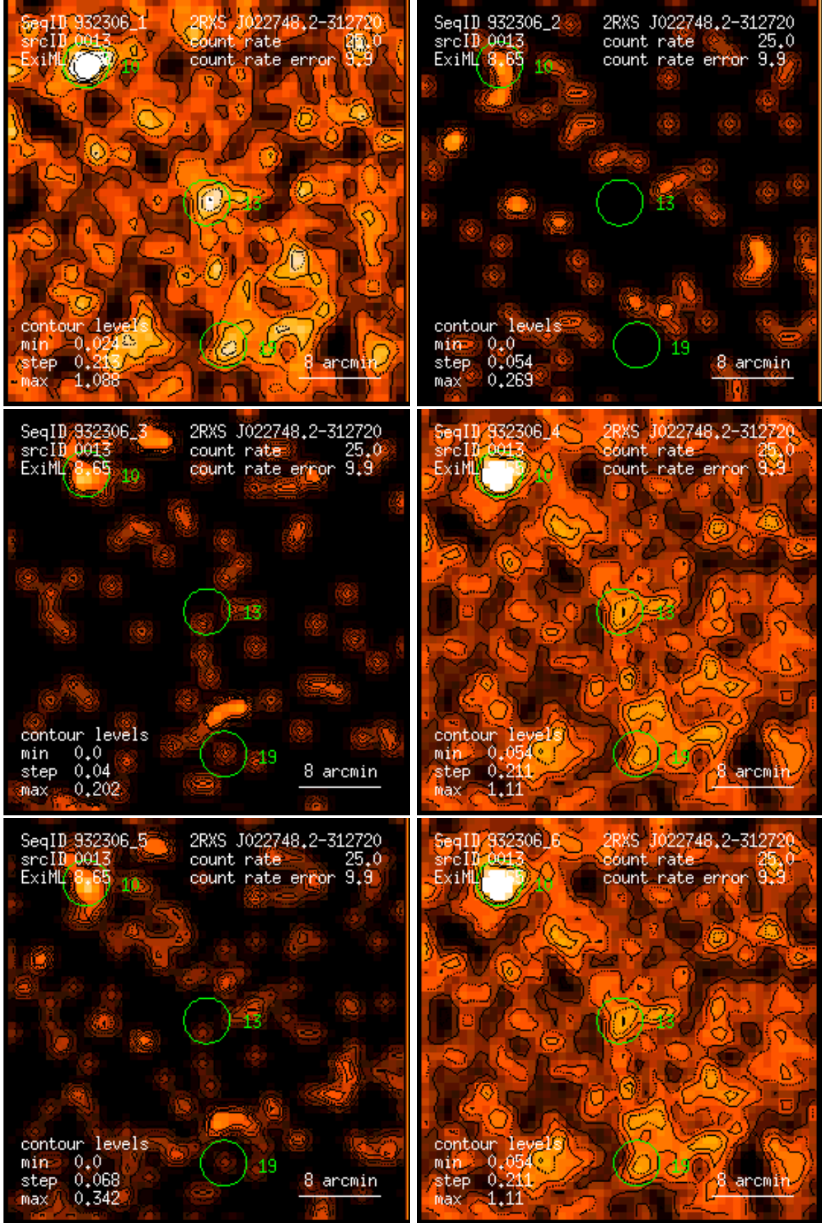
Figure 13: RASS 932306: detection 0013: band rate images, Gaussian filter: (1) PSPC channels 11 – 41, (2) 52 – 90, (3) 91 – 201, (4) 11 – 235, (5) 52 – 201, (6) 11 – 201. Broad band rates in counts/ks. Band rate contour levels in counts/ks/arcmin 2 .
