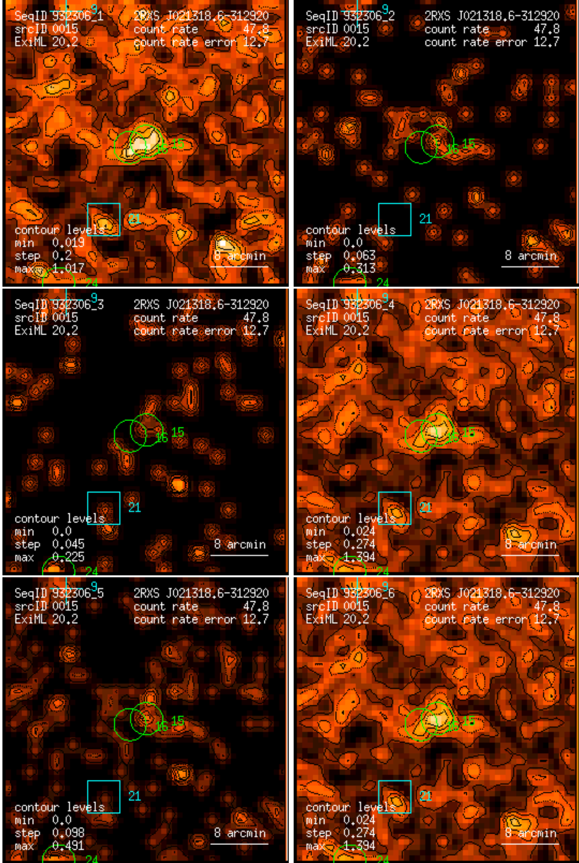
Figure 15: RASS 932306: detection 0015: band rate images, Gaussian filter: (1) PSPC channels 11 – 41, (2) 52 – 90, (3) 91 – 201, (4) 11 – 235, (5) 52 – 201, (6) 11 – 201. Broad band rates in counts/ks. Band rate contour levels in counts/ks/arcmin 2 .
