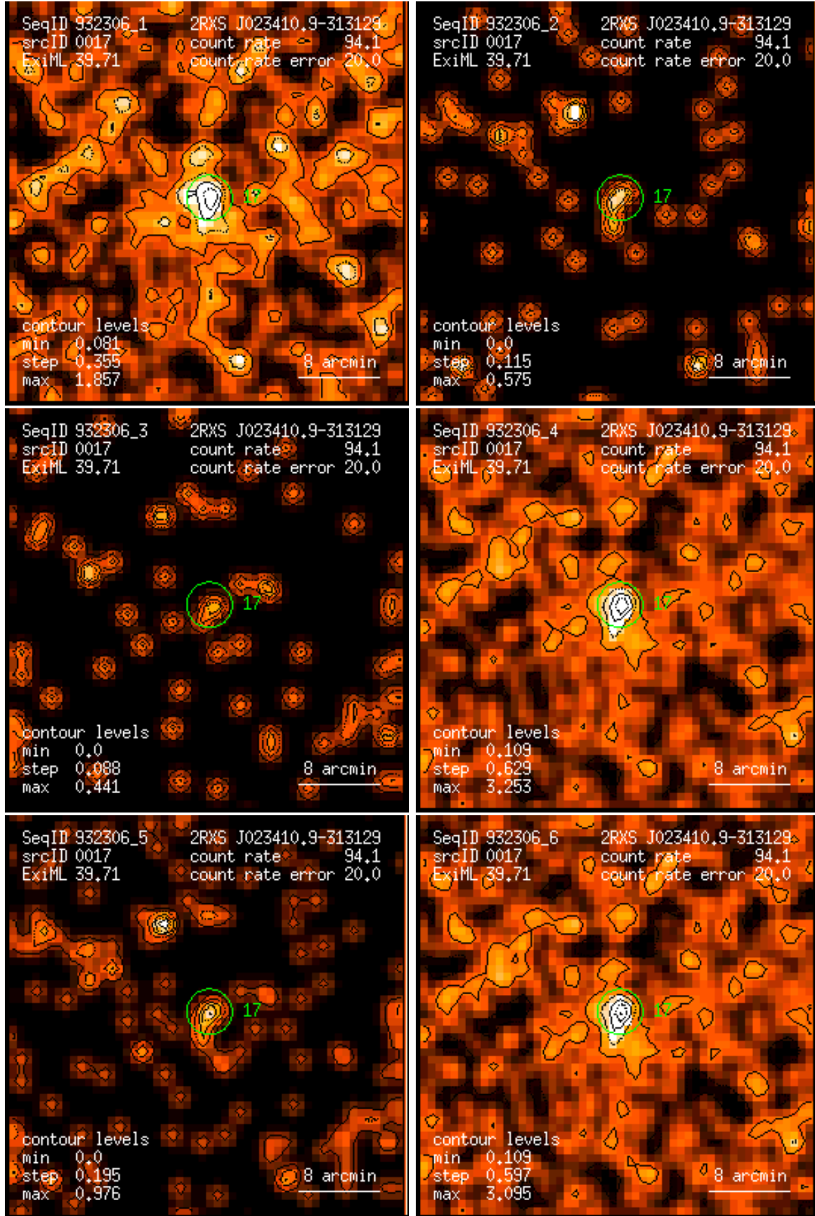
Figure 17: RASS 932306: detection 0017: band rate images, Gaussian filter: (1) PSPC channels 11 – 41, (2) 52 – 90, (3) 91 – 201, (4) 11 – 235, (5) 52 – 201, (6) 11 – 201. Broad band rates in counts/ks. Band rate contour levels in counts/ks/arcmin 2 .
