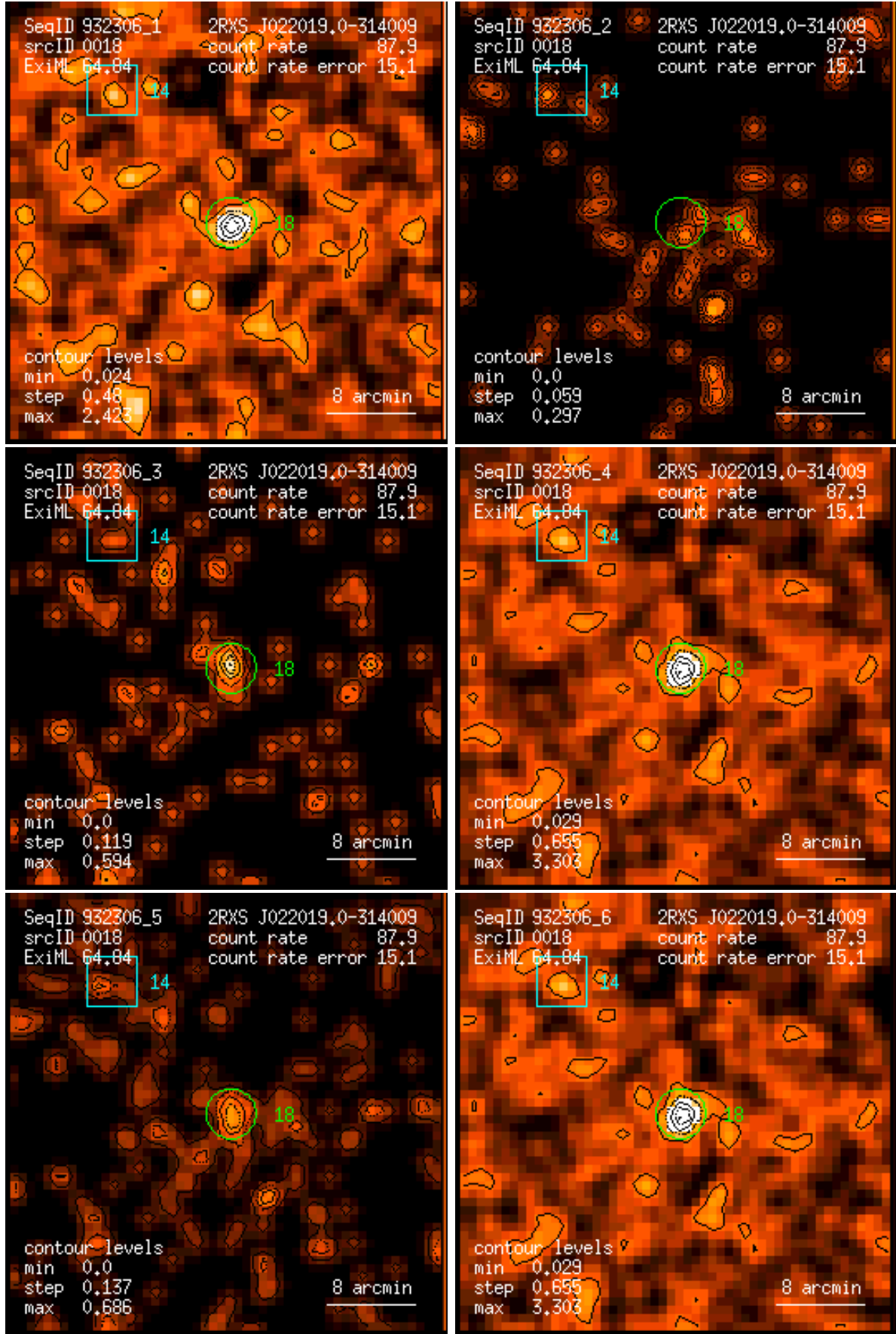
Figure 18: RASS 932306: detection 0018: band rate images, Gaussian filter: (1) PSPC channels 11 – 41, (2) 52 – 90, (3) 91 – 201, (4) 11 – 235, (5) 52 – 201, (6) 11 – 201. Broad band rates in counts/ks. Band rate contour levels in counts/ks/arcmin 2 .
