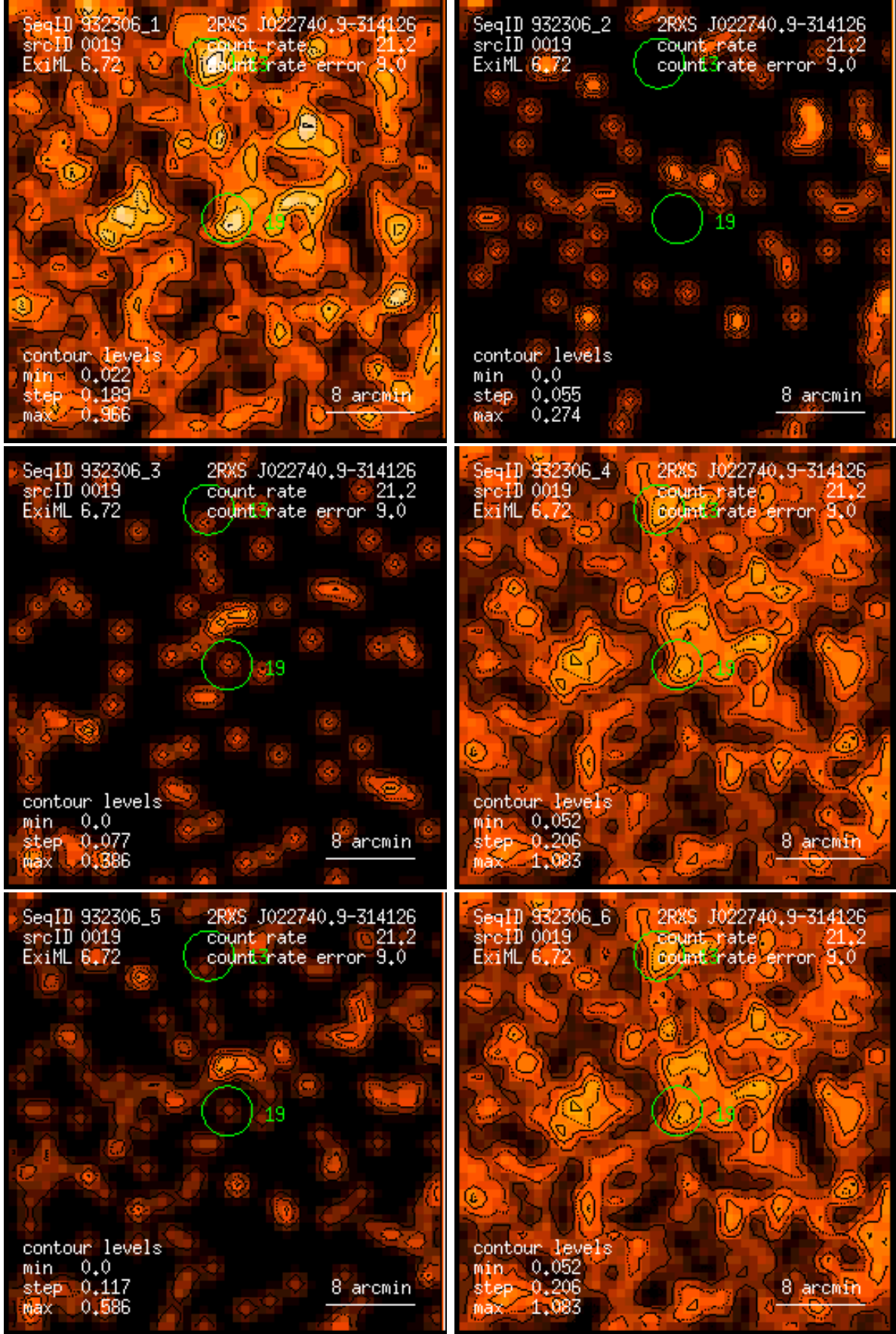
Figure 19: RASS 932306: detection 0019: band rate images, Gaussian filter: (1) PSPC channels 11 – 41, (2) 52 – 90, (3) 91 – 201, (4) 11 – 235, (5) 52 – 201, (6) 11 – 201. Broad band rates in counts/ks. Band rate contour levels in counts/ks/arcmin 2 .
