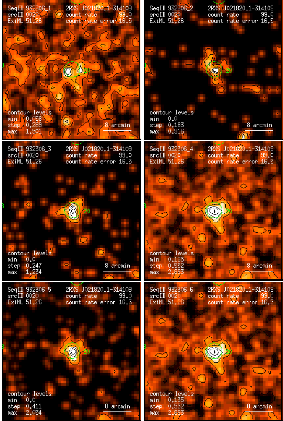
Figure 20: RASS 932306: detection 0020: band rate images, Gaussian filter: (1) PSPC channels 11 – 41, (2) 52 – 90, (3) 91 – 201, (4) 11 – 235, (5) 52 – 201, (6) 11 – 201. Broad band rates in counts/ks. Band rate contour levels in counts/ks/arcmin 2 .
